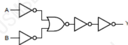
Figure 3. Logic diagram
