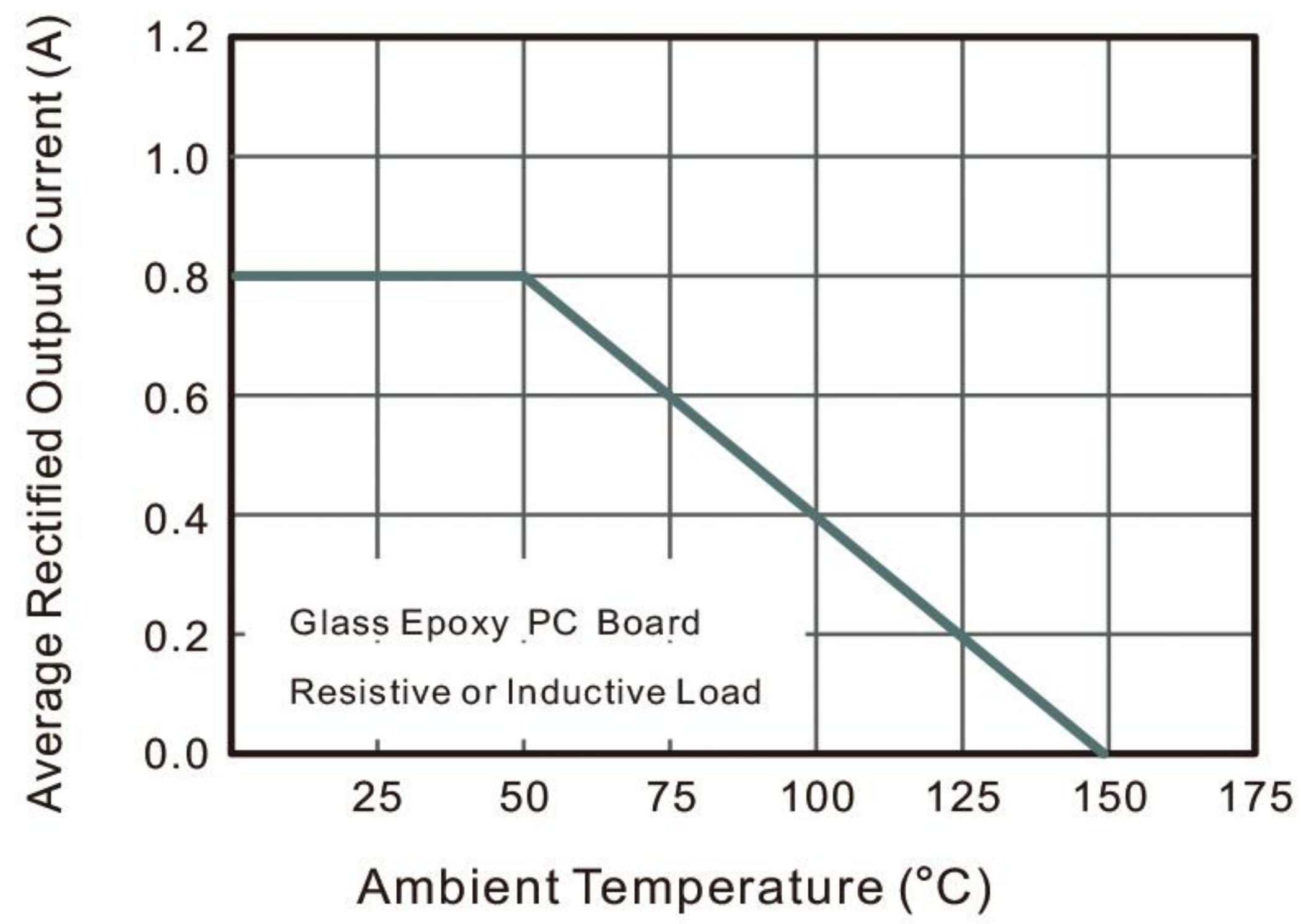
Fig.1 Average Rectified Output Current Derating Curve
