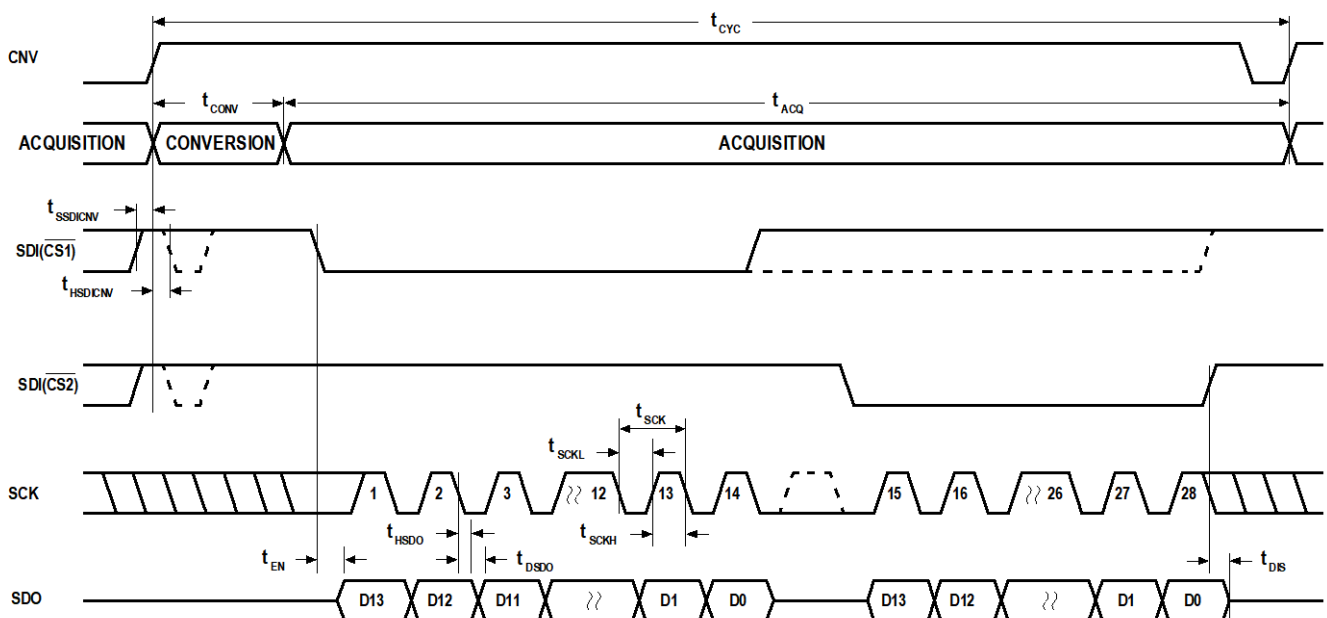
Figure 42. \overline{CS} Mode (4-Wire without Busy Indication) Serial Interface Timing
