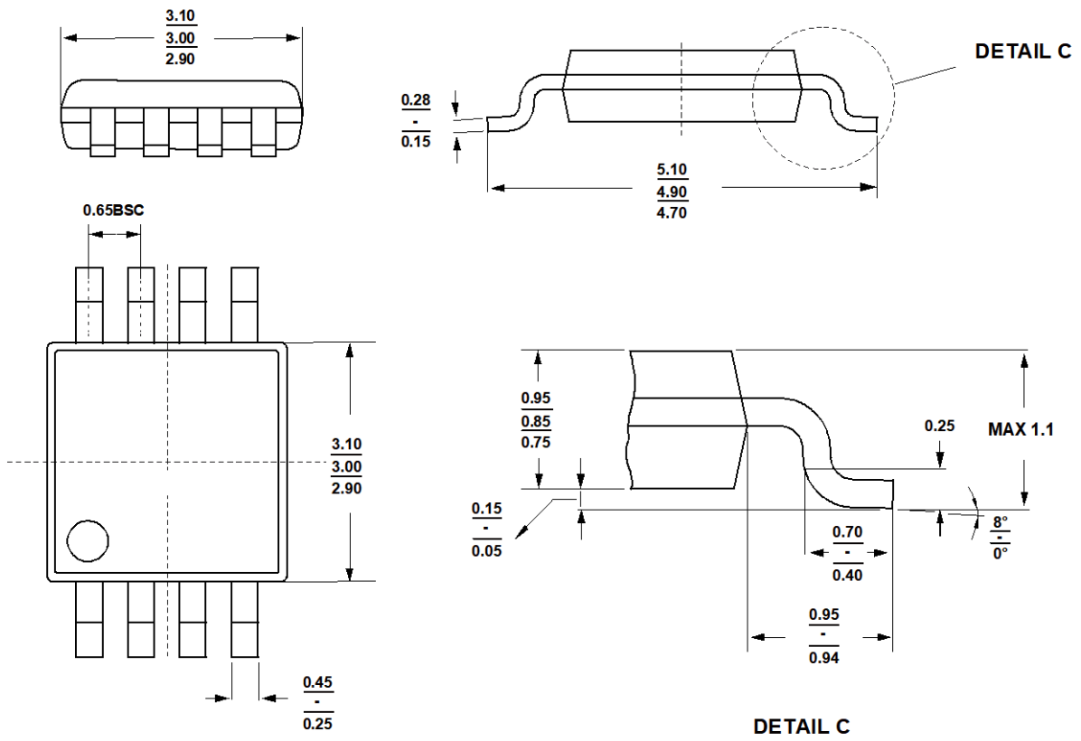
Figure 52. 8-Lead MSOP Package Dimensions Shown in Millimeter
