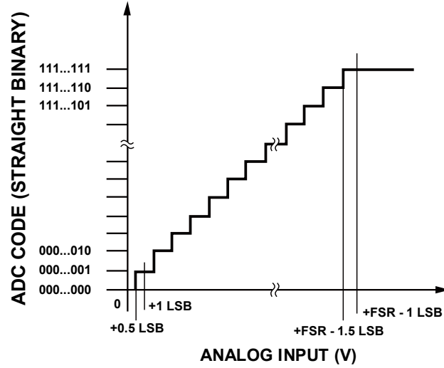
Figure 27. ADC Ideal Transfer Function
