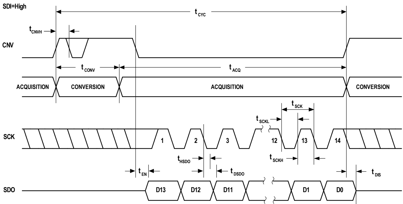
Figure 38. \overline{CS} Mode (3-Wire without Busy Indication) Serial Interface Timing
