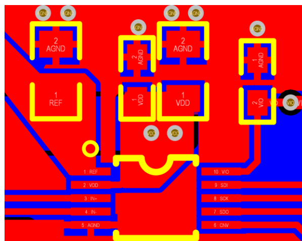
Figure 49. Example Layout and Routing of ZJC2017
