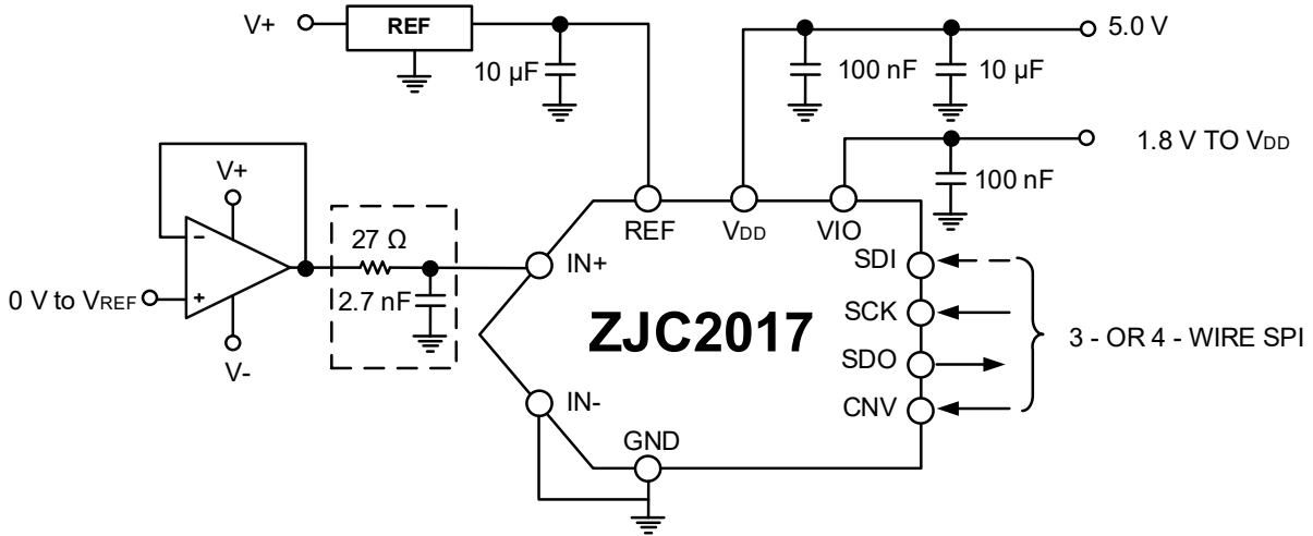
Figure 28. Application Circuits Using Multiple Power Supplies
