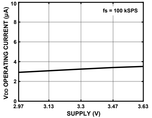
Figure 21. V_{IO} Operating Current vs. Power Supply Voltage
