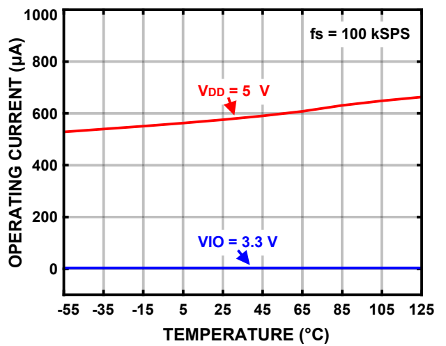
Figure 25. Operating Current vs. Temperature
