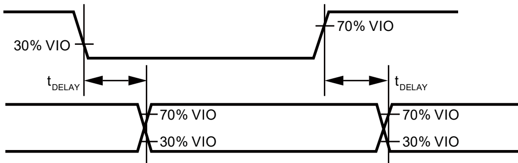
Figure 7. Voltage Levels for Timing
