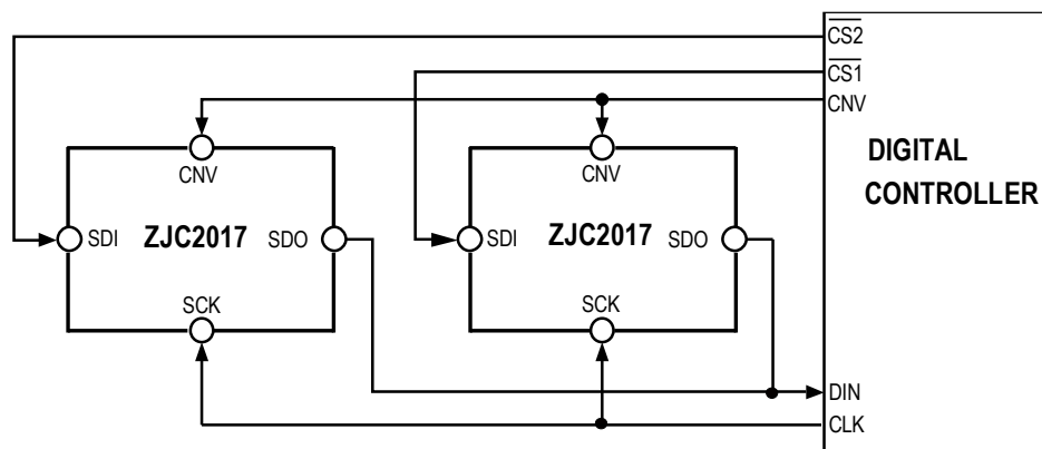
Figure 41. \overline{CS} Mode (4-wire without Busy Indication) Connection Diagram
