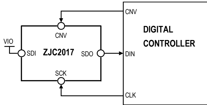
Figure 37. \overline{CS} Mode (3-wire without Busy Indication) Connection Diagram
