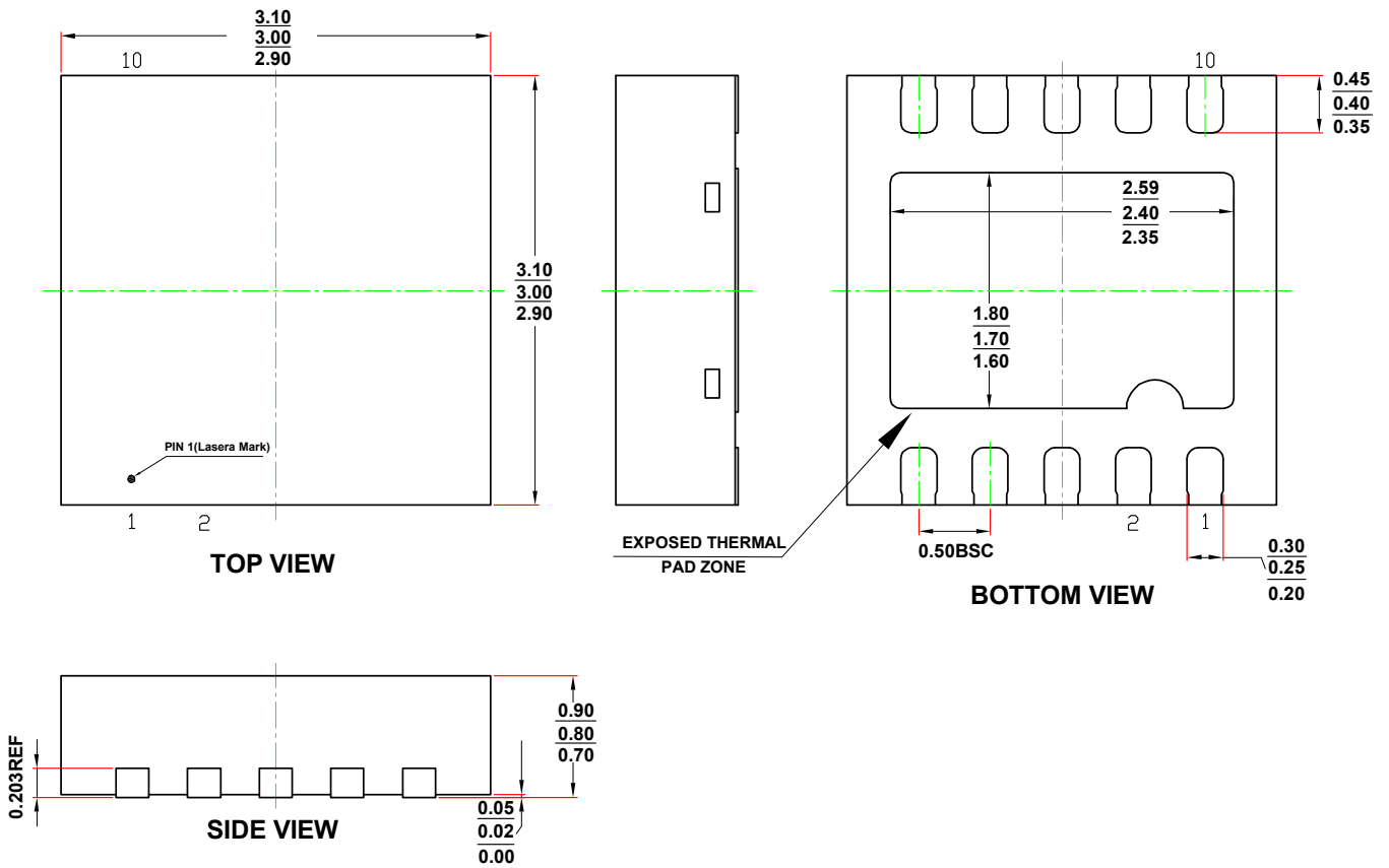
Figure 51. 10-Lead DFN Package Dimensions Shown in Millimeter
