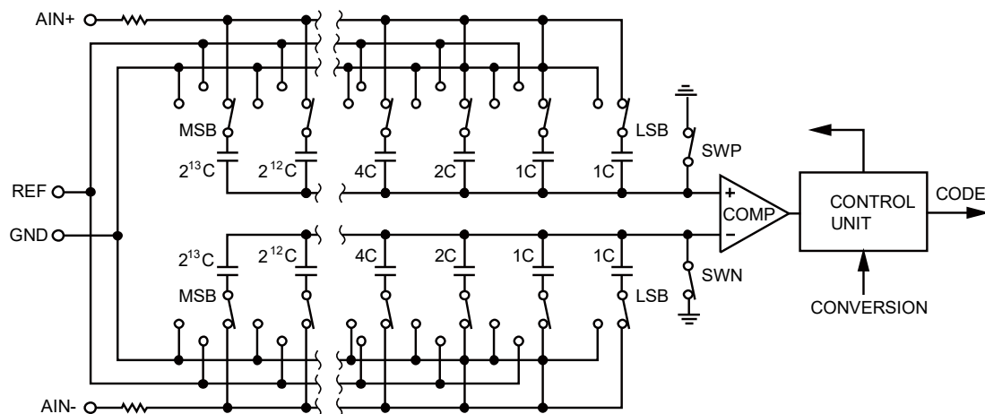
Figure 26. ADC Simplified Circuit Diagram
