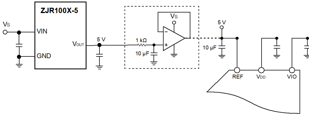
Figure 34. ZJC2017 Reference Pin Drive
