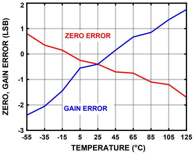
Figure 22. Zero Input, Gain Error vs. Temperature
