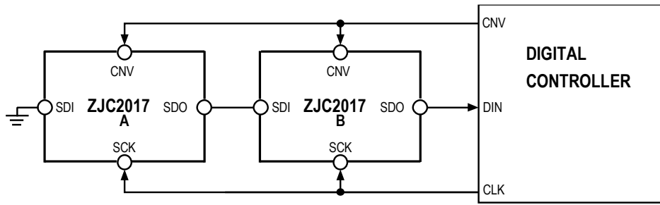
Figure 45. Chain Mode (without Busy Indication) Connection Diagram
