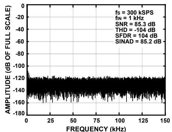
Figure 2. AC Characteristics
