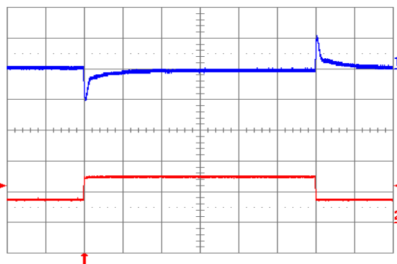
Fig. 1.8V.12: Output voltage response to load current step-change (3.75A – 7.5A – 3.75A) at V_{in} = 24\text{V} . Top trace: output voltage (100 mV/div.). Bottom trace: load current (5 A/div.). Current slew rate: 5 A/µs. C_o = 450\text{ }\mu\text{F} tantalum + 1 µF ceramic. Time scale: 0.2 ms/div.
