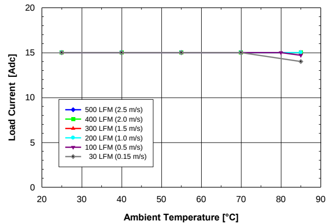
Fig. 2.0V.4: Available load current vs. ambient air temperature and airflow rates for SQ24S15020 converter mounted horizontally with V_{in} = 24V , air flowing from pin 3 to pin 1 and maximum FET temperature \leq 120^{\circ}C .
