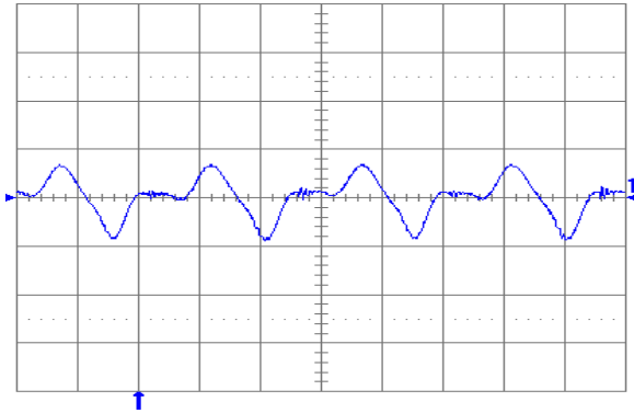
Fig. 1.5V.13: Output voltage ripple (20 mV/div.) at full rated load current into a resistive load with C_o = 10 \mu\text{F} tantalum + 1 \mu\text{F} ceramic and V_{in} = 24 \text{ V} . Time scale: 1 \mu\text{s}/\text{div.}
