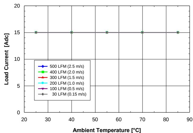
Fig. 1.5V.4: Available load current vs. ambient temperature and airflow rates for SQ24S15015 converter mounted horizontally with V_{in} = 24V , air flowing from pin 3 to pin 1 and maximum FET temperature \leq 120^{\circ}C .
