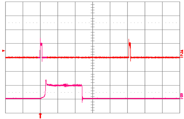
Fig. 2.5V.18: Load current (top trace, 20 \text{ A}/\text{div.} , 20 \text{ ms}/\text{div.} ) into a 10 \text{ m}\Omega short circuit during restart, at V_{in} = 24\text{V} . Bottom trace ( 20 \text{ A}/\text{div.} , 1 \text{ ms}/\text{div.} ) is an expansion of the on-time portion of the top trace.
