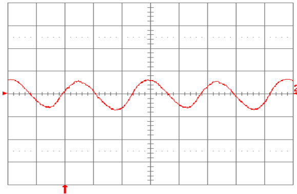
Fig. 6.0V.15: Input reflected ripple current, i_c (100 mA/div.), measured at input terminals at full rated load current and V_{in} = 24 \text{ V} . Refer to Fig. 6.0V.14 for test setup. Time scale: 1 \mu\text{s}/\text{div.}
