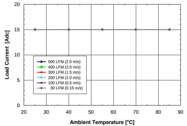
Fig. 1.2V.4: Available load current vs. ambient air temperature and airflow rates for SQ24S15012 converter mounted horizontally with V_{in} = 24V , air flowing from pin 3 to pin 1 and maximum FET temperature \leq 120^{\circ}C .
