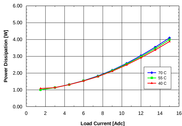
Fig. 1.0V.8: Power dissipation vs. load current and ambient temperature for SQ24T/S15010 converter mounted vertically with V_{in} = 24\text{V} and air flowing from pin 3 to pin 1 at a rate of 200 LFM (1.0 m/s).
