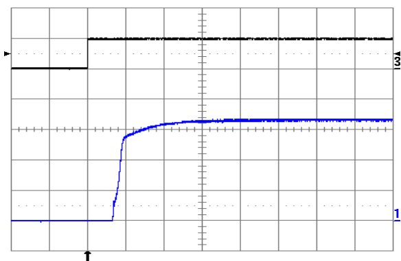
Fig. 3.3V.9: Turn-on transient at full rated load current (resistive) with no output capacitor at V_{in} = 24\text{V} , triggered via ON/OFF pin. Top trace: ON/OFF signal (5 V/div.). Bottom trace: output voltage (1 V/div.). Time scale: 2 ms/div.
