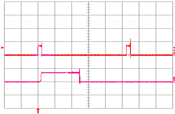
Fig. 6.0V.18: Load current (top trace, 20 \text{ A}/\text{div.} , 20 \text{ ms}/\text{div.} ) into a 10 \text{ m}\Omega short circuit during restart, at V_{in} = 24 \text{ V} . Bottom trace ( 20 \text{ A}/\text{div.} , 2 \text{ ms}/\text{div.} ) is an expansion of the on-time portion of the top trace.
