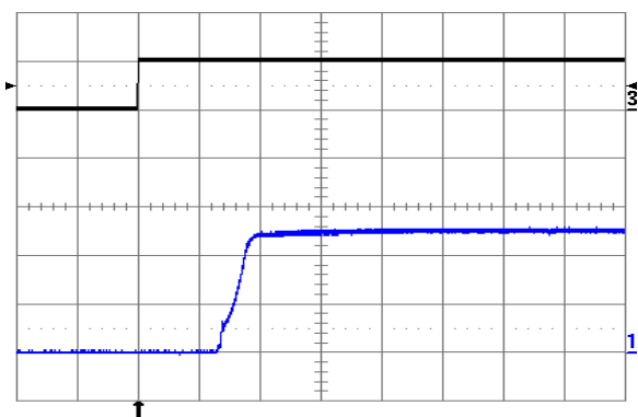
Fig. 2.5V.9: Turn-on transient at full rated load current (resistive) with no output capacitor at V_{in} = 24\text{V} , triggered via ON/OFF pin. Top trace: ON/OFF signal (5 V/div.). Bottom trace: output voltage (1 V/div.). Time scale: 1 ms/div.
