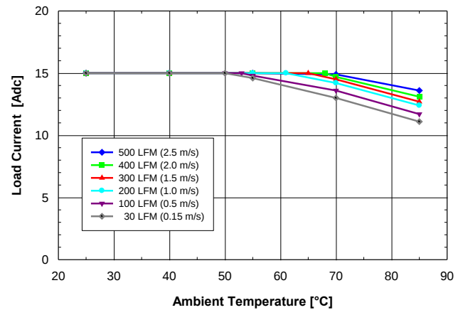
Fig. 3.3V.4: Available load current vs. ambient air temperature and airflow rates for SQ24S15033 converter mounted horizontally with V_{in} = 24V , air flowing from pin 3 to pin 1 and maximum FET temperature \leq 120^{\circ}C .
