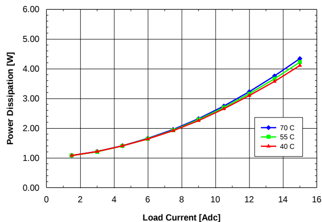
Fig. 1.2V.8: Power dissipation vs. load current and ambient temperature for SQ24T/S15012 converter mounted vertically with V_{in} = 24\text{V} and air flowing from pin 3 to pin 1 at a rate of 200 LFM (1.0 m/s).
