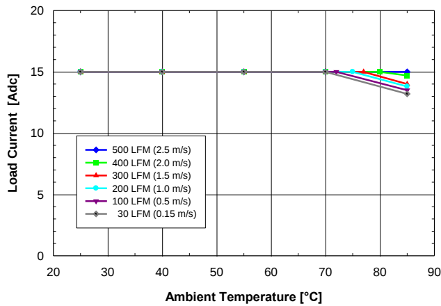
Fig. 2.0V.3: Available load current vs. ambient air temperature and airflow rates for SQ24S15020 converter mounted vertically with V_{in} = 24V , air flowing from pin 3 to pin 1 and maximum FET temperature \leq 120^{\circ}C .
