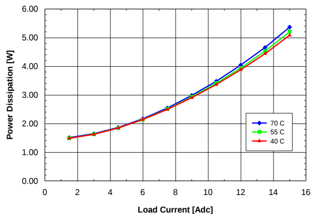
Fig. 2.0V.8: Power dissipation vs. load current and ambient temperature for SQ24T/S15020 converter mounted vertically with V_{in} = 24\text{V} and air flowing from pin 3 to pin 1 at a rate of 200 LFM (1.0 m/s).
