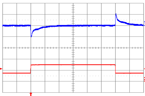
Fig. 3.3V.12: Output voltage response to load current step-change (3.75A – 7.5A – 3.75A) at V_{in} = 24\text{V} . Top trace: output voltage (100 mV/div.). Bottom trace: load current (5 A/div.). Current slew rate: 5 A/ \mu\text{s} . C_o = 450\text{ }\mu\text{F} tantalum + 1 \mu\text{F} ceramic. Time scale: 0.2 ms/div.
