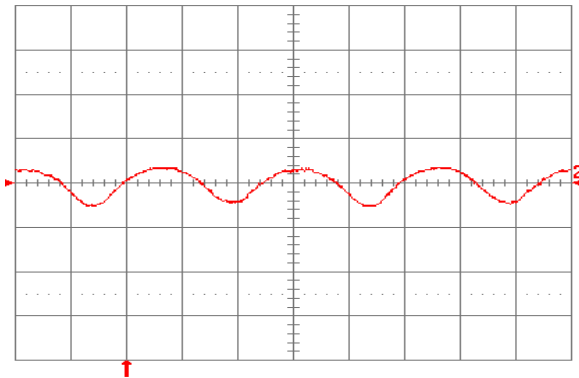
Fig. 1.2V.15: Input reflected ripple current, i_c (100 mA/div.), measured at input terminals at full rated load current and V_{in} = 24 \text{ V} . Refer to Fig. 1.2V.14 for test setup. Time scale: 1 \mu\text{s}/\text{div} .
