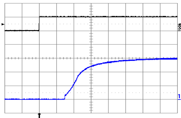
Fig. 6.0V.9: Turn-on transient at full rated load current (resistive) with no output capacitor at V_{in} = 24\text{V} , triggered via ON/OFF pin. Top trace: ON/OFF signal (5 V/div.). Bottom trace: output voltage (2 V/div.). Time scale: 1 ms/div.
