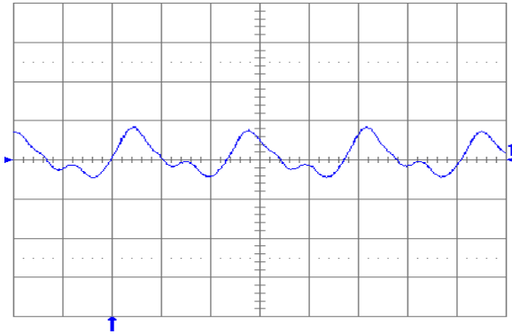
Fig. 3.3V.13: Output voltage ripple (20 mV/div.) at full rated load current into a resistive load with C_o = 10 \mu\text{F} tantalum + 1 \mu\text{F} ceramic and V_{in} = 24 \text{ V} . Time scale: 1 \mu\text{s}/\text{div} .
