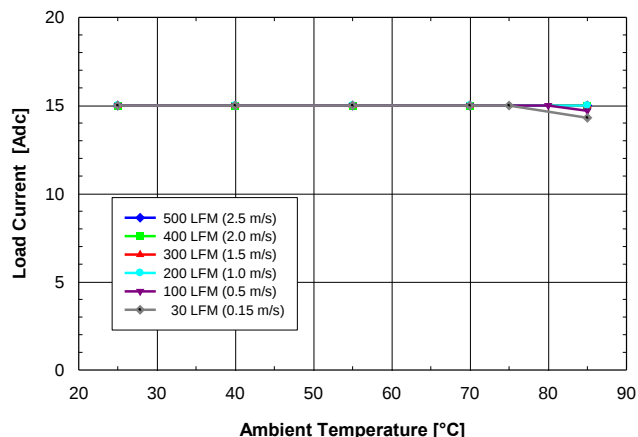
Fig. 1.8V.1: Available load current vs. ambient air temperature and airflow rates for SQ24T15018 converter with B height pins mounted vertically with V_{in} = 24V , air flowing from pin 3 to pin 1 and maximum FET temperature \leq 120^{\circ}C .
