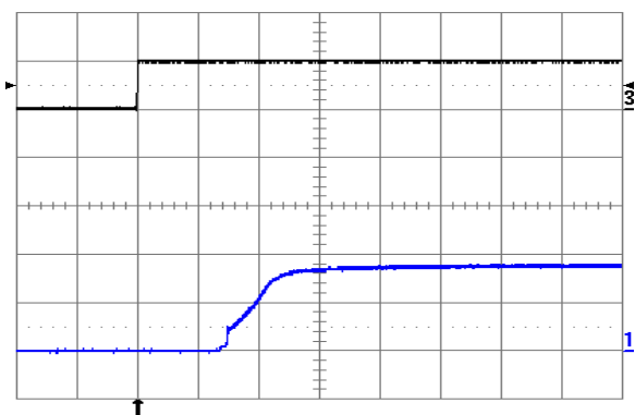
Fig. 1.8V.9: Turn-on transient at full rated load current (resistive) with no output capacitor at V_{in} = 24\text{V} , triggered via ON/OFF pin. Top trace: ON/OFF signal (5 V/div.). Bottom trace: output voltage (1 V/div.). Time scale: 1 ms/div.
