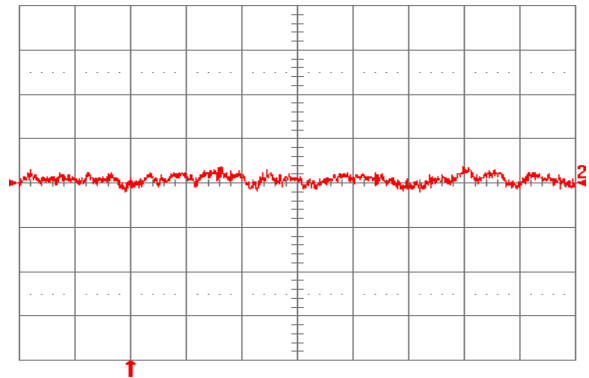
Fig. 1.0V.16: Input reflected ripple current, i_s (10 mA/div.), measured through 10 \mu\text{H} at the source at full rated load current and V_{in} = 24 \text{ V} . Refer to Fig. 1.0V.14 for test setup. Time scale: 1 \mu\text{s}/\text{div} .
