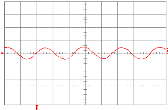
Fig. 2.5V.15: Input reflected ripple current, i_c (100 mA/div.), measured at input terminals at full rated load current and V_{in} = 24\text{V} . Refer to Fig. 2.5V.14 for test setup. Time scale: 1 \mu\text{s}/\text{div} .
