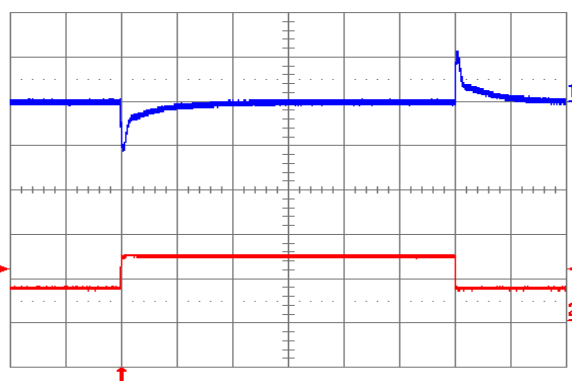
Fig. 1.0V.12: Output voltage response to load current step-change (3.75 A – 7.5 A – 3.75 A) at V_{in} = 24\text{V} . Top trace: output voltage (100 mV/div.). Bottom trace: load current (5 A/div.). Current slew rate: 5 A/µs. C_o = 450\text{ }\mu\text{F} tantalum + 1 µF ceramic. Time scale: 0.2 ms/div.
