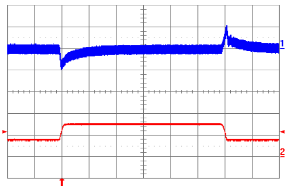
Fig. 2.5V.11: Output voltage response to load current step-change (3.75 A – 7.5 A – 3.75 A) at V_{in} = 24\text{V} . Top trace: output voltage (100 mV/div.). Bottom trace: load current (5 A/div.). Current slew rate: 0.1 A/ \mu\text{s} . C_o = 1\text{ }\mu\text{F} ceramic. Time scale: 0.2 ms/div.
