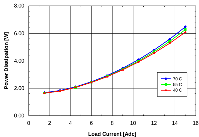
Fig. 2.5V.8: Power dissipation vs. load current and ambient temperature for SQ24T/S15025 converter mounted vertically with V_{in} = 24\text{V} and air flowing from pin 3 to pin 1 at a rate of 200 LFM (1.0 m/s).
