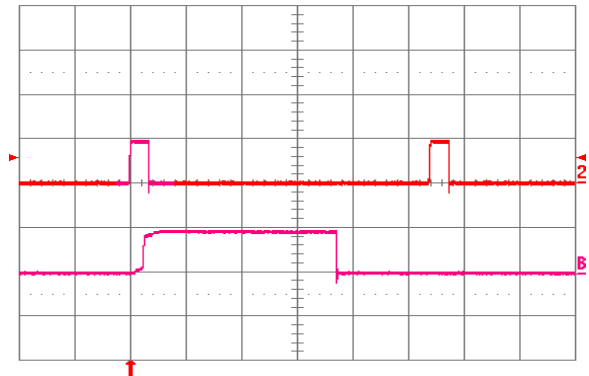
Fig. 1.0V.18: Load current (top trace, 20 \text{ A}/\text{div.} , 20 \text{ ms}/\text{div.} ) into a 10 \text{ m}\Omega short circuit during restart, at V_{in} = 24 \text{ V} . Bottom trace ( 20 \text{ A}/\text{div.} , 2 \text{ ms}/\text{div.} ) is an expansion of the on-time portion of the top trace.
