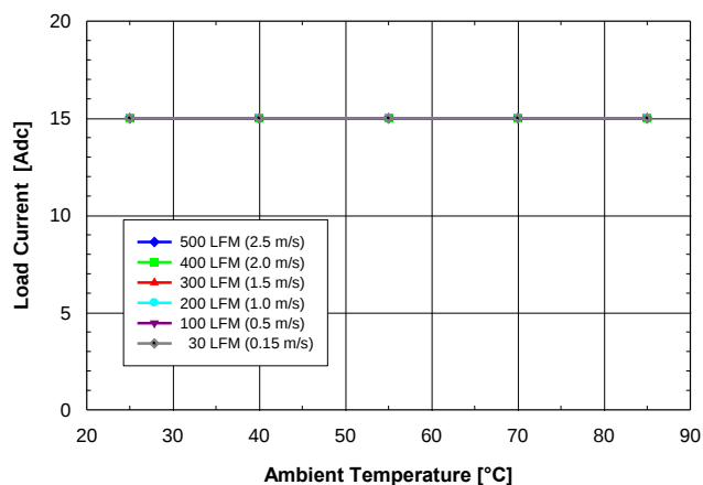
Fig. 1.0V.3: Available load current vs. ambient air temperature and airflow rates for SQ24S15010 converter mounted vertically with V_{in} = 24V , air flowing from pin 3 to pin 1 and maximum FET temperature \leq 120^{\circ}C .
