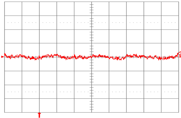
Fig. 6.0V.16: Input reflected ripple current, i_s (10 mA/div.), measured through 10 \mu\text{H} at the source at full rated load current and V_{in} = 24 \text{ V} . Refer to Fig. 6.0V.14 for test setup. Time scale: 1 \mu\text{s}/\text{div.}
