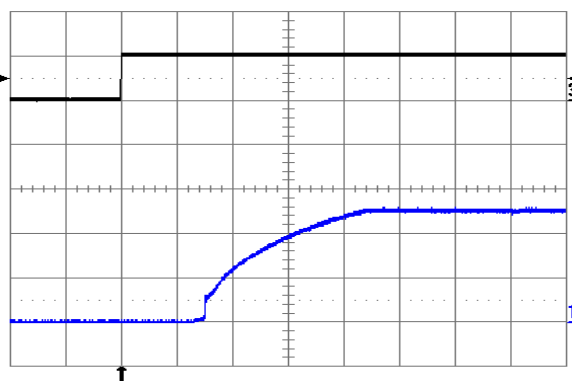
Fig. 2.5V.10: Turn-on transient at full rated load current (resistive) plus 10,000 \mu\text{F} at V_{in} = 24\text{V} , triggered via ON/OFF pin. Top trace: ON/OFF signal (5 V/div.). Bottom trace: output voltage (1 V/div.). Time scale: 1 ms/div.
