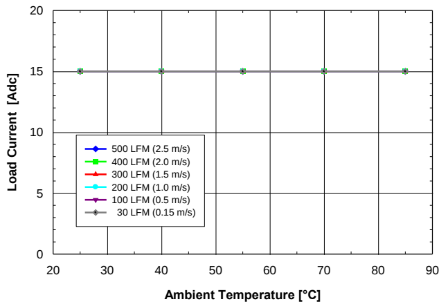
Fig. 1.2V.3: Available load current vs. ambient air temperature and airflow rates for SQ24S15012 converter mounted vertically with V_{in} = 24V , air flowing from pin 3 to pin 1 and maximum FET temperature \leq 120^{\circ}C .
