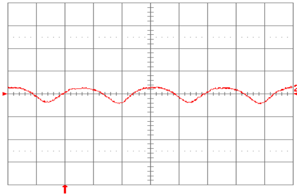
Fig. 1.0V.15: Input reflected ripple current, i_c (100 mA/div.), measured at input terminals at full rated load current and V_{in} = 24 \text{ V} . Refer to Fig. 1.0V.14 for test setup. Time scale: 1 \mu\text{s}/\text{div} .
