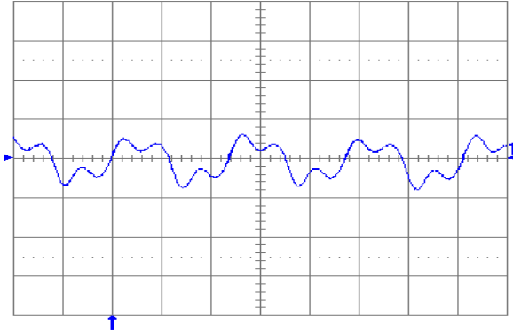
Fig. 2.5V.13: Output voltage ripple (20 mV/div.) at full rated load current into a resistive load with C_o = 10 \mu\text{F} tantalum + 1\mu\text{F} ceramic and V_{in} = 24 \text{ V} . Time scale: 1 \mu\text{s}/\text{div} .
