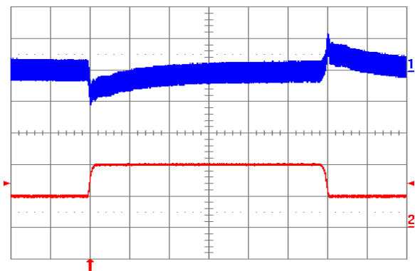
Fig. 6.0V.11: Output voltage response to load current step-change (2A - 4A - 2A) at V_{in} = 24\text{V} . Top trace: output voltage (100mV/div.). Bottom trace: load current (2A/div.). Current slew rate: 0.1 A/µs. C_o = 1\text{ }\mu\text{F} ceramic. Time scale: 0.2 ms/div.
