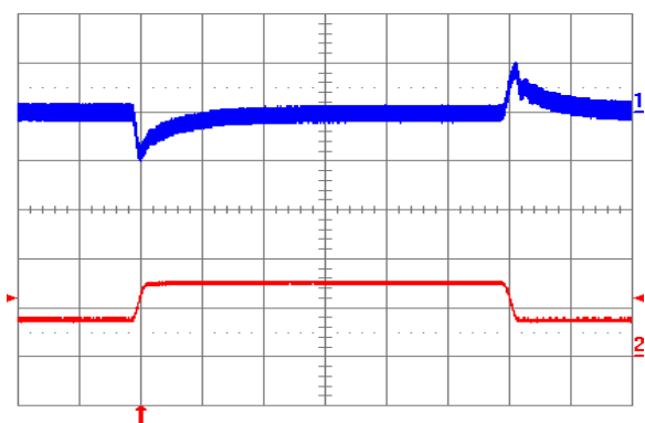
Fig. 1.5V.11: Output voltage response to load current step-change (3.75 A – 7.5 A – 3.75 A) at V_{in} = 24\text{V} . Top trace: output voltage (100 mV/div.). Bottom trace: load current (5 A/div.). Current slew rate: 0.1 A/ \mu\text{s} . C_o = 1\text{ }\mu\text{F} ceramic. Time scale: 0.2 ms/div.
