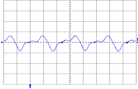
Fig. 1.8V.13: Output voltage ripple (20 mV/div.) at full rated load current into a resistive load with C_o = 10 \mu\text{F} tantalum + 1\mu\text{F} ceramic and V_{in} = 24 \text{ V} . Time scale: 1 \mu\text{s}/\text{div} .
