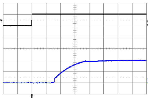
Fig. 2.0V.10: Turn-on transient at full rated load current (resistive) plus 10,000µF at V_{in} = 24\text{V} , triggered via ON/OFF pin. Top trace: ON/OFF signal (5 V/div.). Bottom trace: output voltage (1 V/div.). Time scale: 1 ms/div.
