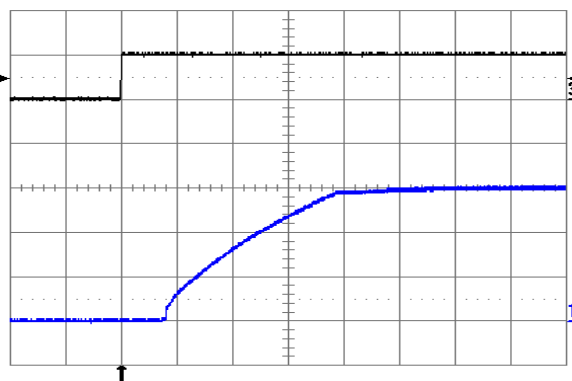
Fig. 6.0V.10: Turn-on transient at full rated load current (resistive) plus 10,000µF at V_{in} = 24\text{V} , triggered via ON/OFF pin. Top trace: ON/OFF signal (5 V/div.). Bottom trace: output voltage (2 V/div.). Time scale: 2 ms/div.
