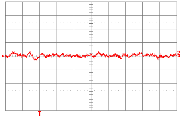
Fig. 2.5V.16: Input reflected ripple current, i_s (10 mA/div.), measured through 10 \mu\text{H} at the source at full rated load current and V_{in} = 24\text{V} . Refer to Fig. 2.5V.14 for test setup. Time scale: 1 \mu\text{s}/\text{div} .
