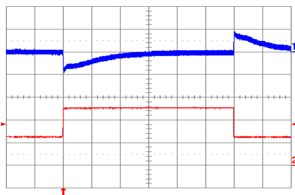
Fig. 5.0V.12: Output voltage response to load current step-change (2.5A – 5A – 2.5A) at V_{in} = 24\text{V} . Top trace: output voltage (100 mV/div.). Bottom trace: load current (2 A/div.). Current slew rate: 5 A/ \mu\text{s} . C_o = 450 \mu\text{F} tantalum + 1 \mu\text{F} ceramic. Time scale: 0.2 ms/div.
