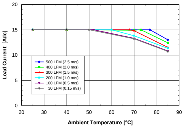
Fig. 3.3V.3: Available load current vs. ambient air temperature and airflow rates for SQ24S15033 converter mounted vertically with V_{in} = 24V , air flowing from pin 3 to pin 1 and maximum FET temperature \leq 120^{\circ}C .
