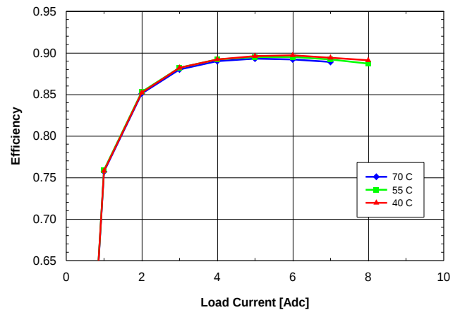
Fig. 6.0V.6: Efficiency vs. load current and ambient temperature for SQ24T/S08060 converter mounted vertically with V_{in} = 24V and air flowing from pin 3 to pin 1 at a rate of 200 LFM (1.0 m/s).
