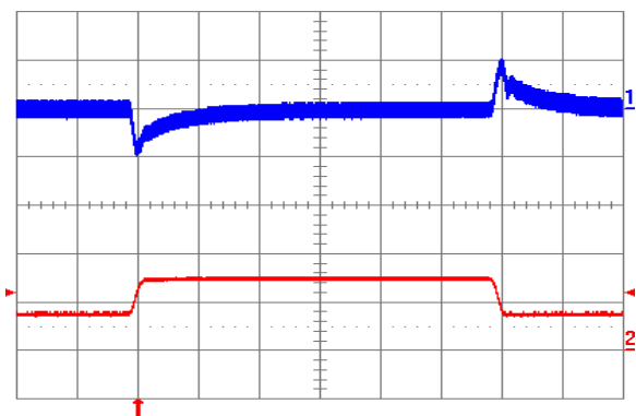
Fig. 1.2V.11: Output voltage response to load current step-change (3.75 A – 7.5 A – 3.75 A) at V_{in} = 24\text{V} . Top trace: output voltage (100 mV/div.). Bottom trace: load current (5 A/div.). Current slew rate: 0.1 A/ \mu\text{s} . C_o = 1\text{ }\mu\text{F} ceramic. Time scale: 0.2 ms/div.
