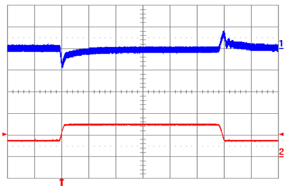
Fig. 1.8V.11: Output voltage response to load current step-change (3.75A – 7.5A – 3.75A) at V_{in} = 24\text{V} . Top trace: output voltage (100 mV/div.). Bottom trace: load current (5 A/div.). Current slew rate: 0.1 A/µs. C_o = 1\text{ }\mu\text{F} ceramic. Time scale: 0.2 ms/div.
