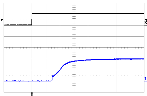
Fig. 2.0V.9: Turn-on transient at full rated load current (resistive) with no output capacitor at V_{in} = 24\text{V} , triggered via ON/OFF pin. Top trace: ON/OFF signal (5 V/div.). Bottom trace: output voltage (1 V/div.). Time scale: 1 ms/div.
