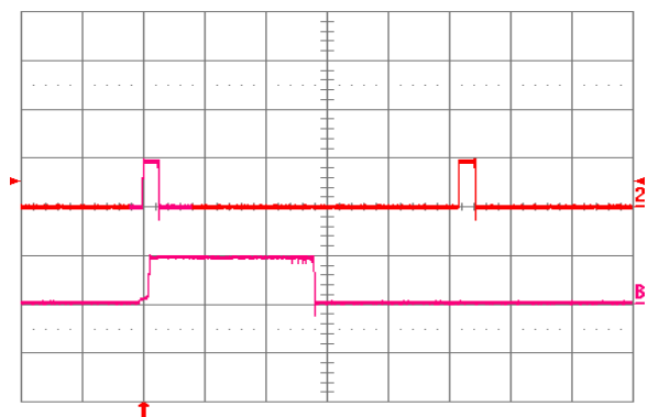
Fig. 1.5V.18: Load current (top trace, 20 \text{ A}/\text{div.} , 20 \text{ ms}/\text{div.} ) into a 10 \text{ m}\Omega short circuit during restart, at V_{in} = 24 \text{ V} . Bottom trace ( 20 \text{ A}/\text{div.} , 2 \text{ ms}/\text{div.} ) is an expansion of the on-time portion of the top trace.
