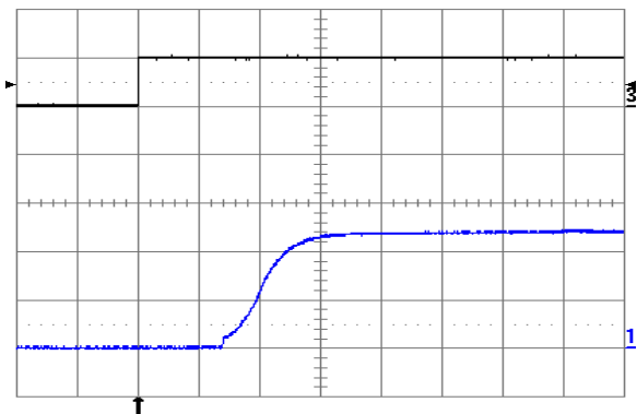
Fig. 12V.9: Turn-on transient at full rated load current (resistive) with no output capacitor at V_{in} = 24\text{V} , triggered via ON/OFF pin. Top trace: ON/OFF signal (5 V/div.). Bottom trace: output voltage (5 V/div.). Time scale: 1 ms/div.
