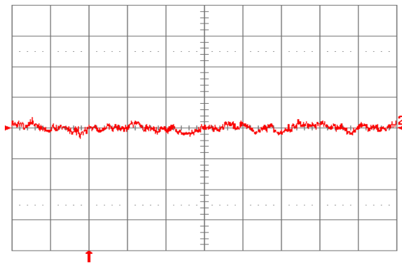
Fig. 2.0V.16: Input reflected ripple current, i_s (10 mA/div.), measured through 10 \mu\text{H} at the source at full rated load current and V_{in} = 24 \text{ V} . Refer to Fig. 2.0V.14 for test setup. Time scale: 1 \mu\text{s}/\text{div.}
