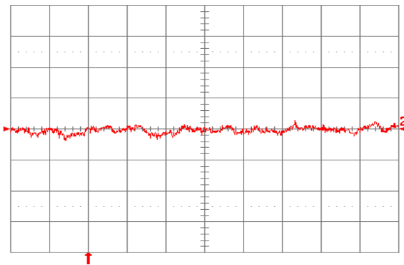
Fig. 3.3V.16: Input reflected ripple current, i_s (10 mA/div.), measured through 10 \mu\text{H} at the source at full rated load current and V_{in} = 24 \text{ V} . Refer to Fig. 3.3V.14 for test setup. Time scale: 1 \mu\text{s}/\text{div} .
