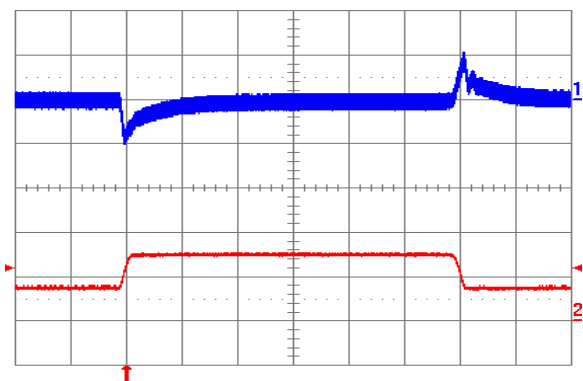
Fig. 2.0V.11: Output voltage response to load current step-change (3.75A – 7.5A – 3.75A) at V_{in} = 24\text{V} . Top trace: output voltage (100 mV/div.). Bottom trace: load current (5 A/div.). Current slew rate: 0.1 A/µs. C_o = 1\text{ }\mu\text{F} ceramic. Time scale: 0.2 ms/div.
