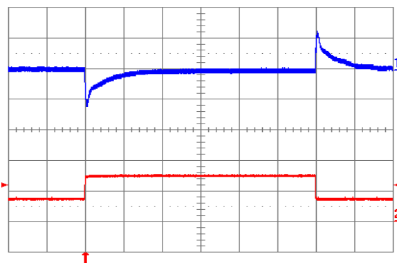
Fig. 2.0V.12: Output voltage response to load current step-change (3.75A – 7.5A – 3.75A) at V_{in} = 24\text{V} . Top trace: output voltage (100 mV/div.). Bottom trace: load current (5 A/div.). Current slew rate: 5 A/µs. C_o = 450\text{ }\mu\text{F} tantalum + 1 µF ceramic. Time scale: 0.2 ms/div.
