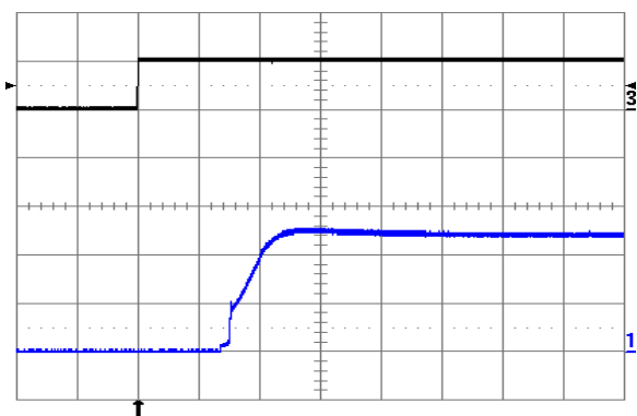
Fig. 1.2V.9: Turn-on transient at full rated load current (resistive) with no output capacitor at V_{in} = 24\text{V} , triggered via ON/OFF pin. Top trace: ON/OFF signal (5 V/div.). Bottom trace: output voltage (0.5 V/div.). Time scale: 1 ms/div.
