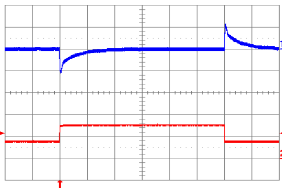
Fig. 2.5V.12: Output voltage response to load current step-change (3.75 A – 7.5 A – 3.75 A) at V_{in} = 24\text{V} . Top trace: output voltage (100 mV/div.). Bottom trace: load current (5 A/div.). Current slew rate: 5 A/ \mu\text{s} . C_o = 450\text{ }\mu\text{F} tantalum + 1 \mu\text{F} ceramic. Time scale: 0.2 ms/div.
