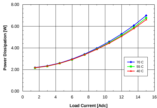
Fig. 3.3V.8: Power dissipation vs. load current and ambient temperature for SQ24T/S15033 converter mounted vertically with V_{in} = 24\text{V} and air flowing from pin 3 to pin 1 at a rate of 200 LFM (1.0 m/s).
