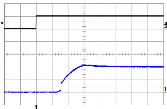
Fig. 1.0V.11: Turn-on transient at full rated load current (resistive) plus 10,000 µF at V_{in} = 24\text{V} , triggered via ON/OFF pin. Top trace: ON/OFF signal (5 V/div.). Bottom trace: output voltage (0.5 V/div.). Time scale: 1 ms/div.
