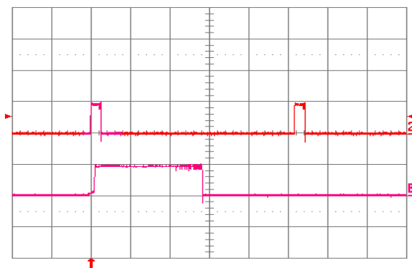
Fig. 2.0V.18: Load current (top trace, 20 \text{ A}/\text{div.} , 20 \text{ ms}/\text{div.} ) into a 10 \text{ m}\Omega short circuit during restart, at V_{in} = 24 \text{ V} . Bottom trace ( 20 \text{ A}/\text{div.} , 2 \text{ ms}/\text{div.} ) is an expansion of the on-time portion of the top trace.
