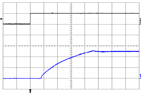
Fig. 5.0V.10: Turn-on transient at full rated load current (resistive) plus 10,000 \mu\text{F} at V_{in} = 24\text{V} , triggered via ON/OFF pin. Top trace: ON/OFF signal (5 V/div.). Bottom trace: output voltage (2 V/div.). Time scale: 2 ms/div.
