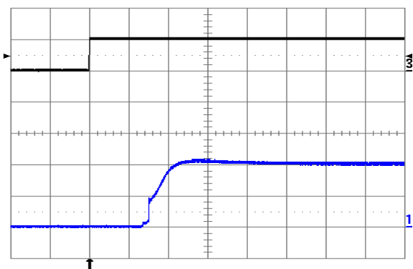
Fig. 1.0V.9: Turn-on transient at full rated load current (resistive) with no output capacitor at V_{in} = 24\text{V} , triggered via ON/OFF pin. Top trace: ON/OFF signal (5 V/div.). Bottom trace: output voltage (0.5 V/div.). Time scale: 1 ms/div.
