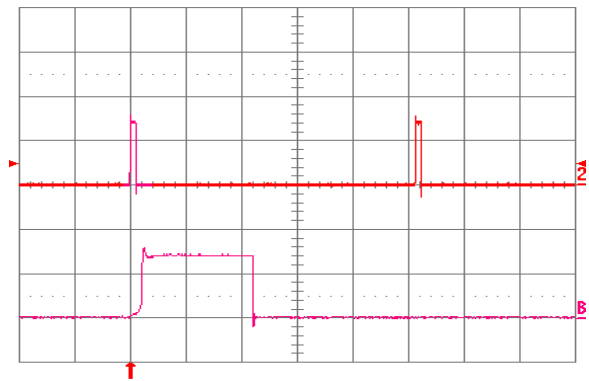
Fig. 5.0V.18: Load current (top trace, 10 \text{ A}/\text{div.} , 20 \text{ ms}/\text{div.} ) into a 10 \text{ m}\Omega short circuit during restart, at V_{in} = 24 \text{ V} . Bottom trace ( 10 \text{ A}/\text{div.} , 1 \text{ ms}/\text{div.} ) is an expansion of the on-time portion of the top trace.
