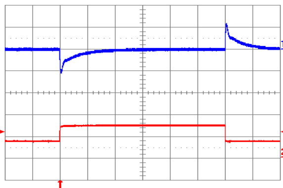
Fig. 1.2V.12: Output voltage response to load current step-change (3.75 A – 7.5 A – 3.75 A) at V_{in} = 24\text{V} . Top trace: output voltage (100 mV/div.). Bottom trace: load current (5 A/div.). Current slew rate: 5 A/ \mu\text{s} . C_o = 450\text{ }\mu\text{F} tantalum + 1 \mu\text{F} ceramic. Time scale: 0.2 ms/div.
