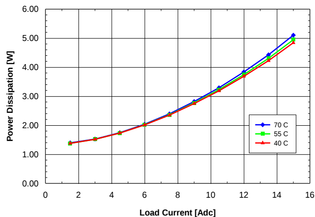
Fig. 1.8V.8: Power dissipation vs. load current and ambient temperature for SQ24T/S15018 converter mounted vertically with V_{in} = 24\text{V} and air flowing from pin 3 to pin 1 at a rate of 200 LFM (1.0 m/s).
