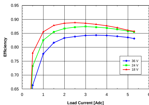
Fig. 8.0V.2: Efficiency vs. load current and input voltage for SQ24T/S05080 converter mounted vertically with air flowing from pin 3 to pin 1 at a rate of 300 LFM (1.5 m/s) and Ta = 25°C.
