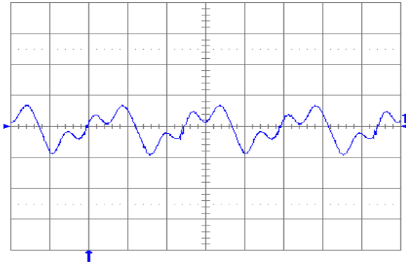
Fig. 2.0V.13: Output voltage ripple (20 mV/div.) at full rated load current into a resistive load with C_o = 10 \mu\text{F} tantalum + 1 \mu\text{F} ceramic and V_{in} = 24 \text{ V} . Time scale: 1 \mu\text{s}/\text{div.}
