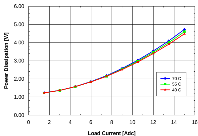
Fig. 1.5V.8: Power dissipation vs. load current and ambient temperature for SQ24T/S15015 converter mounted vertically with V_{in} = 24\text{V} and air flowing from pin 3 to pin 1 at a rate of 200 LFM (1.0 m/s).
