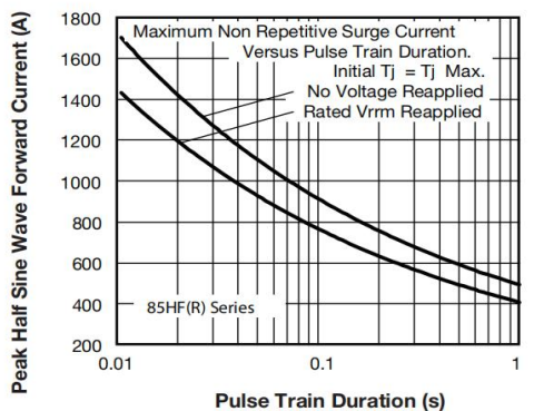
Fig. 10 - Maximum Non-Repetitive Surge Current
