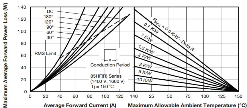
Fig. 8 - Forward Power Loss Characteristics
