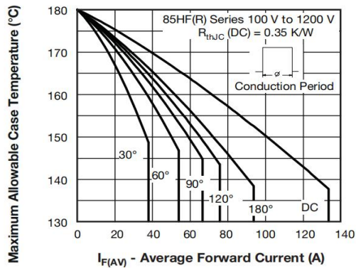
Fig. 2 - Current Ratings Characteristics
