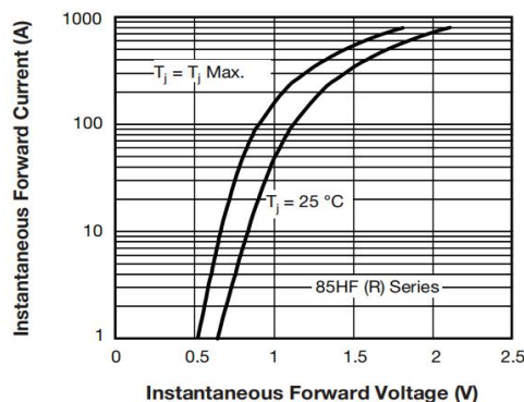
Fig. 12 - Forward Voltage Drop Characteristics (for 1400 V, 1600 V)
