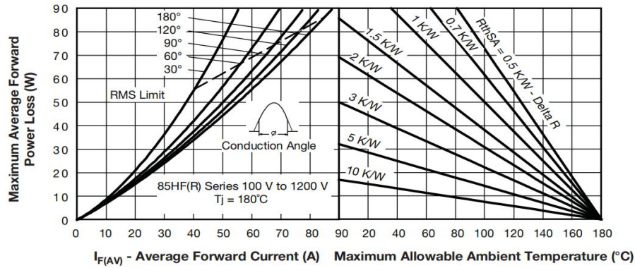
Fig. 5 - Forward Power Loss Characteristics
