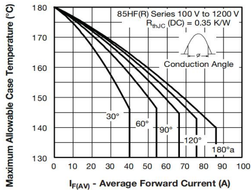
Fig. 1 - Current Ratings Characteristics
