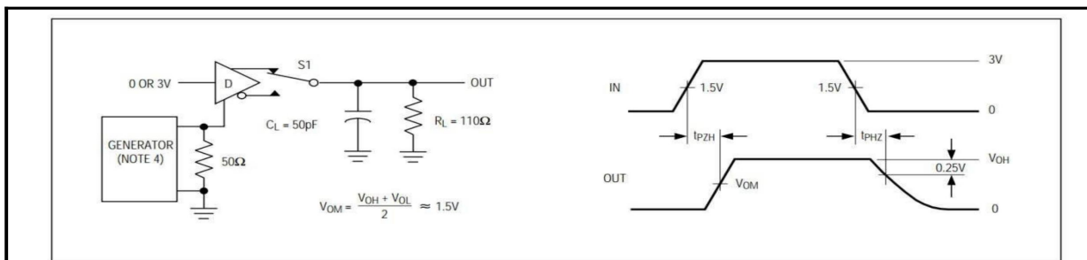
Fig. 5 Driver enable and disable times
