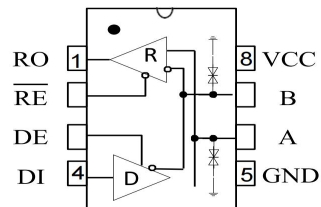
Figure 1 MAX1487ECSA-TD pin configuration
