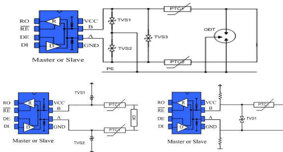
Fig. 11 Port protection scheme
