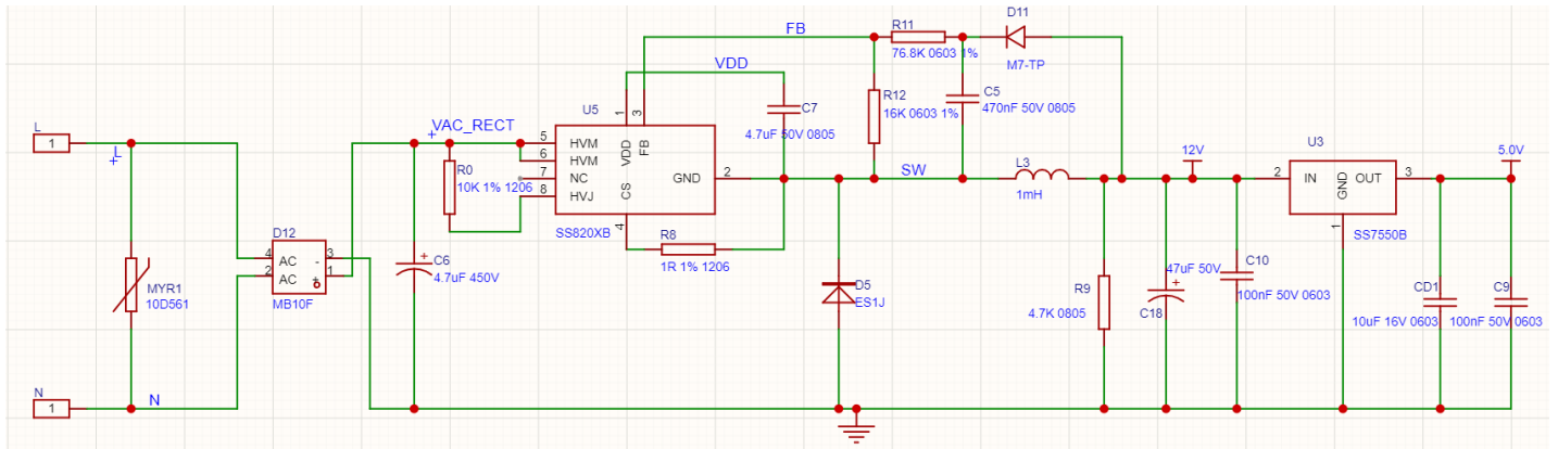
Figure 4. SS8201B Typical Application Circuit
