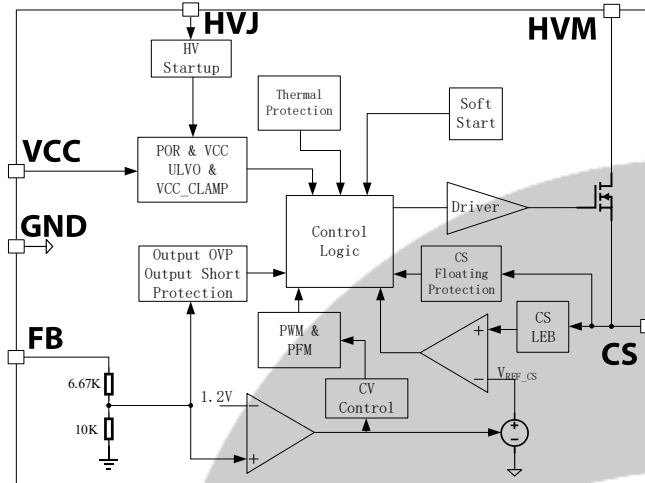
Figure 3. Block Diagram
