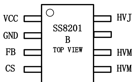
Figure 2. Pin Configuration
