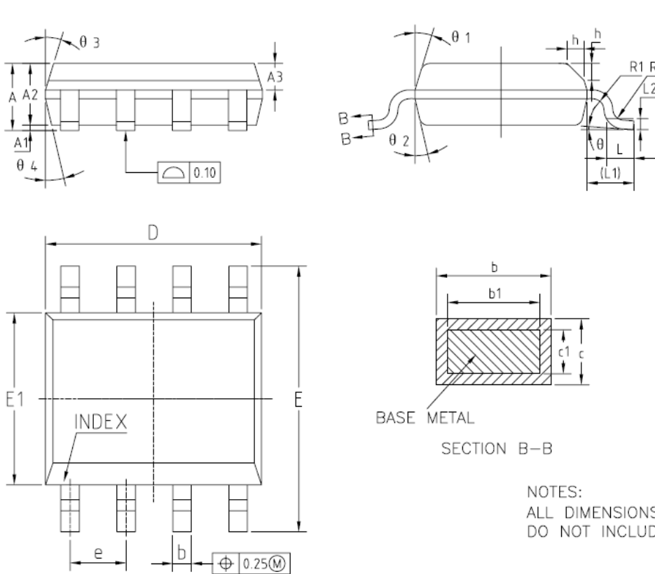
Figure 5. 8-Lead Small Outline Package [SOP]
