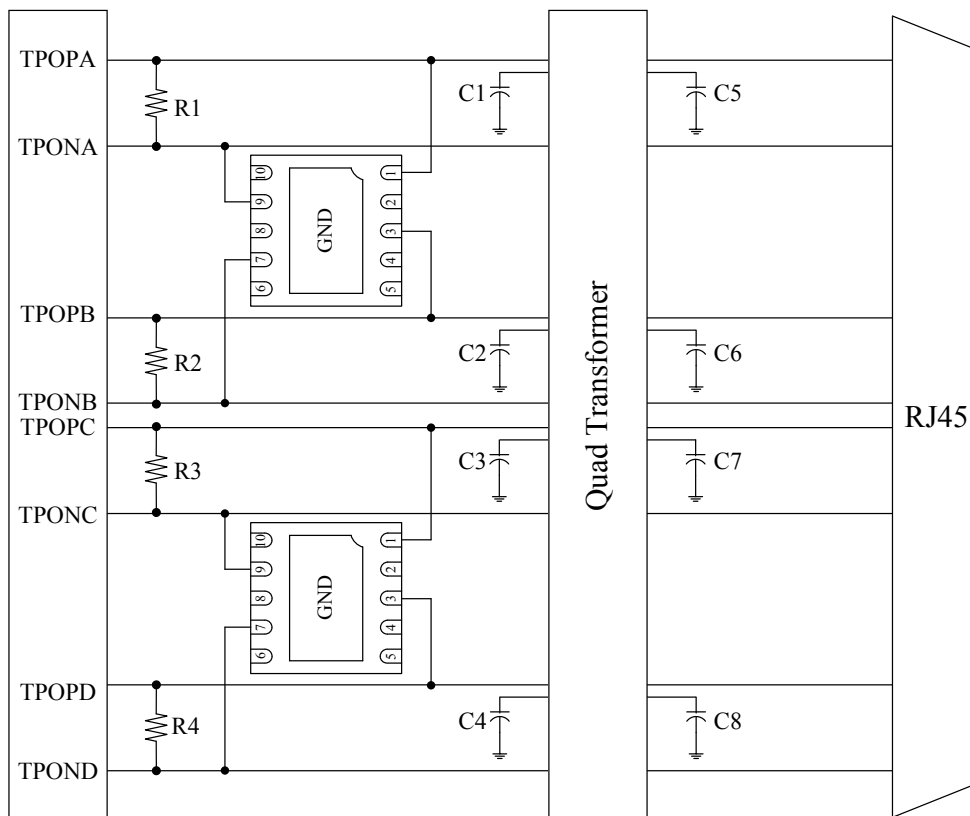
Schematic Diagram for Gigabit Ethernet ESD/Surge Protection using TS3314PRX
