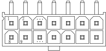
2x7 Pin
