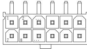
2x6 Pin
