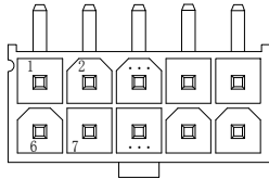
2x5 Pin
