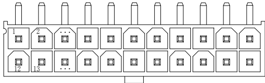
2x11 Pin
