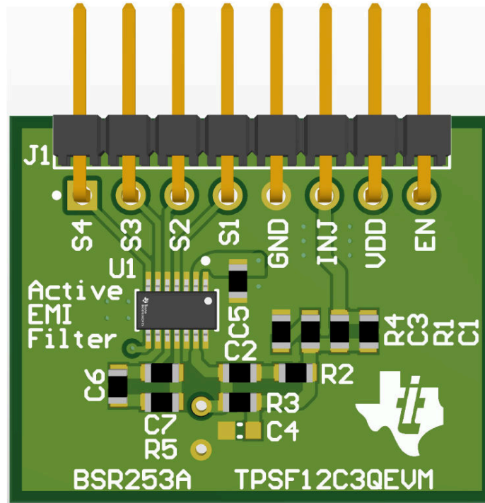
Figure 9-9. Typical Layout
