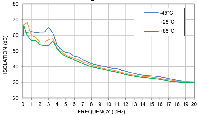
ISOLATION vs. TEMPERATURE, P_{IN} = -25 dBm
