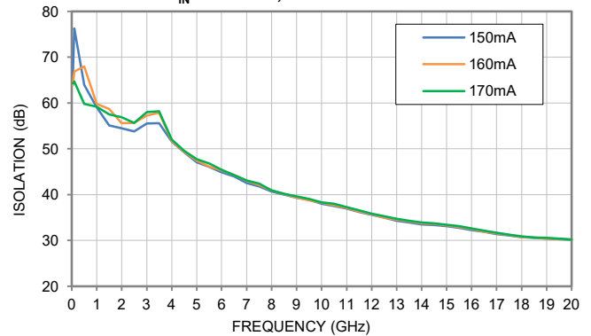
ISOLATION vs. DEVICE CURRENT, P_{IN} = -25 dBm, TEMPERATURE = +25°C
