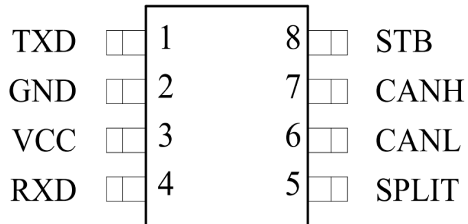
TJA1049T/1 Pin Diagram
