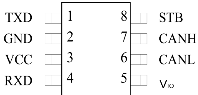
TJA1049T/3 Pin Diagram
