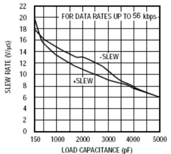
SLEW RATE vs. LOAD CAPACITANCE
