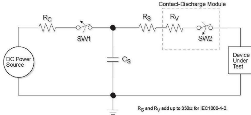
Fig. 2. ESD Test Circuit for IEC1000-4-2
