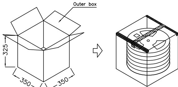
Outer box
