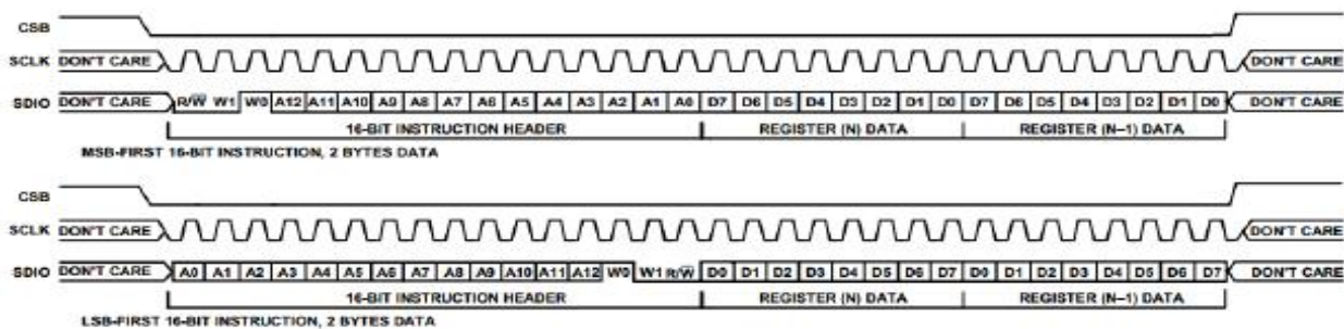
Figure5.3: MSB First and LSB First Instruction and Data Phases
