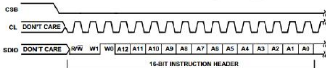
Figure5.2, Instruction Phase Bit Field.
