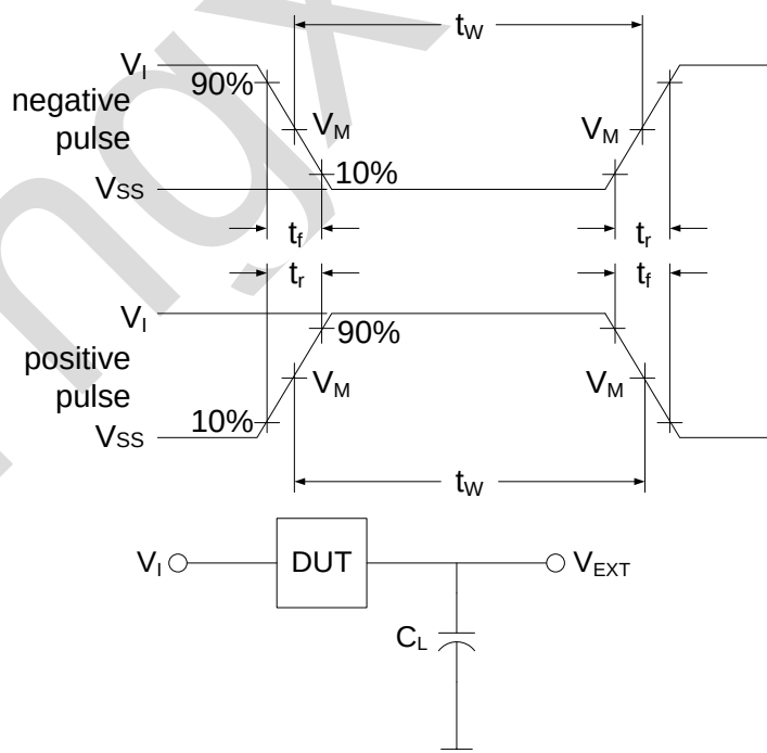
Figure 3. Load circuit
