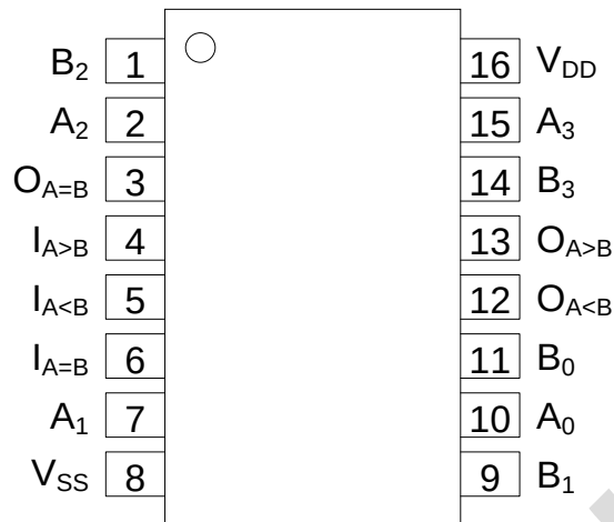
Figure 2. Pin configurations
