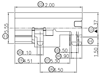
Recommended pcb layout (top view) (thickness=1.2±0.10mm) (tolerance ±0.05)
