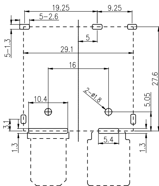
PCB Layout
