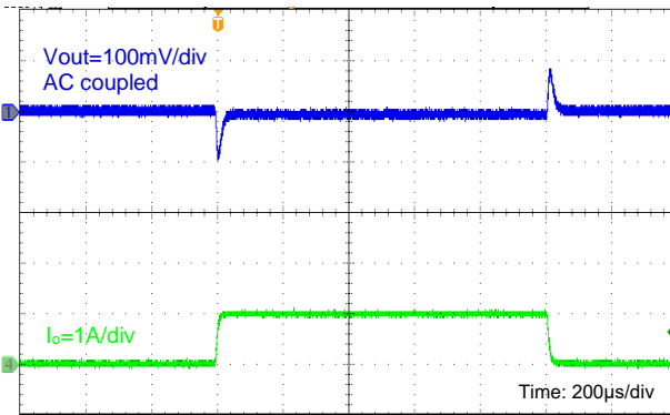
Load Transient
