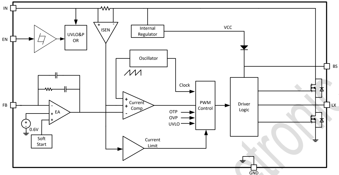
Figure 2. TMI3281 Block Diagram
