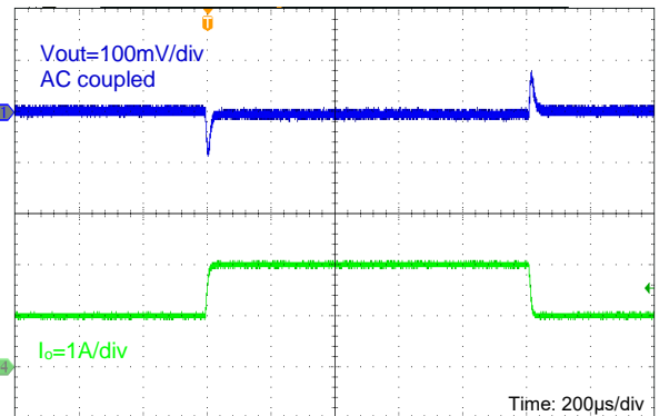
Load Transient
