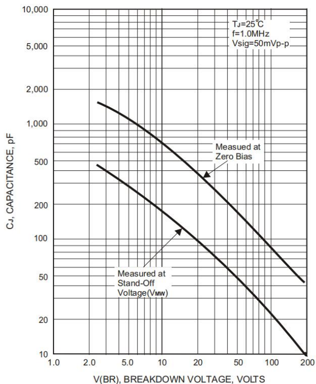
FIG.4-TYPICAL JUNCTION CAPACITANCE
