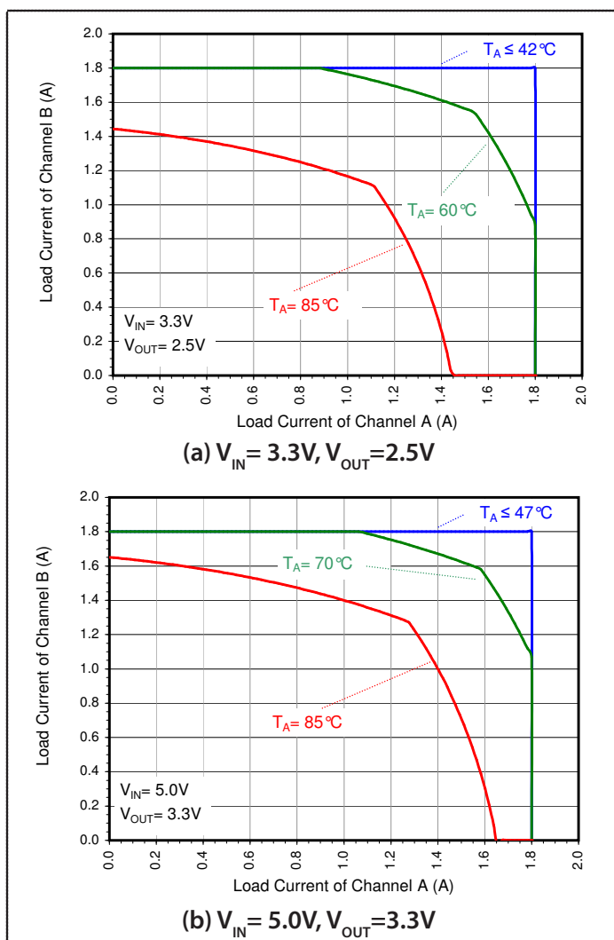
Figure 3 — Maximum allowable Load Current for each channel for a maximum junction temperature of 125°C
