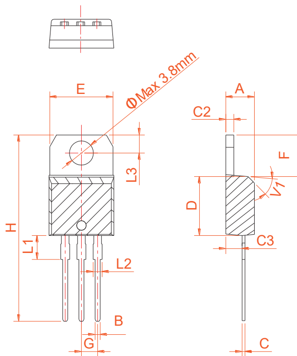
TO-220B Non-Ins
