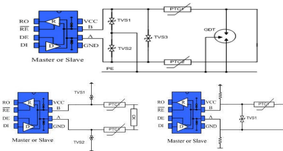
Fig. 11 Port protection scheme
