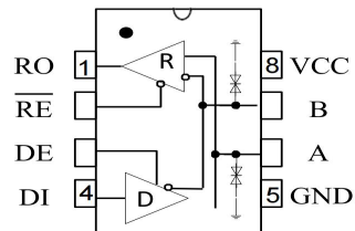
Figure 1 MAX483EESA-TD pin configuration
