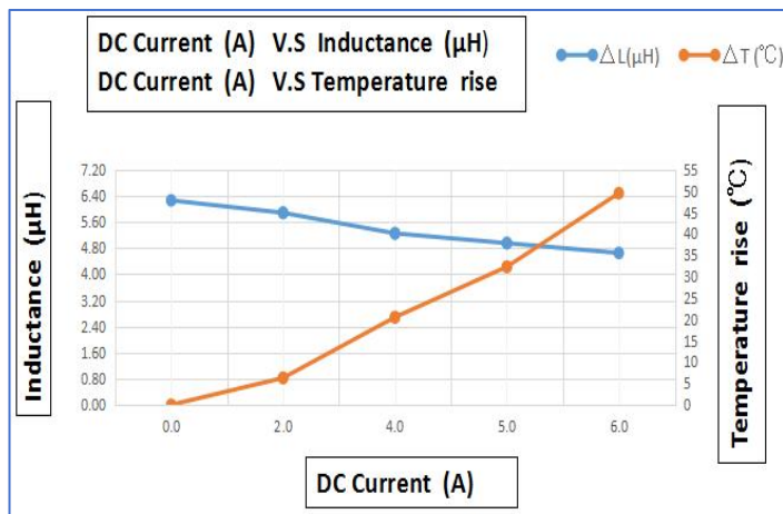
GSM0630-6R8-M
