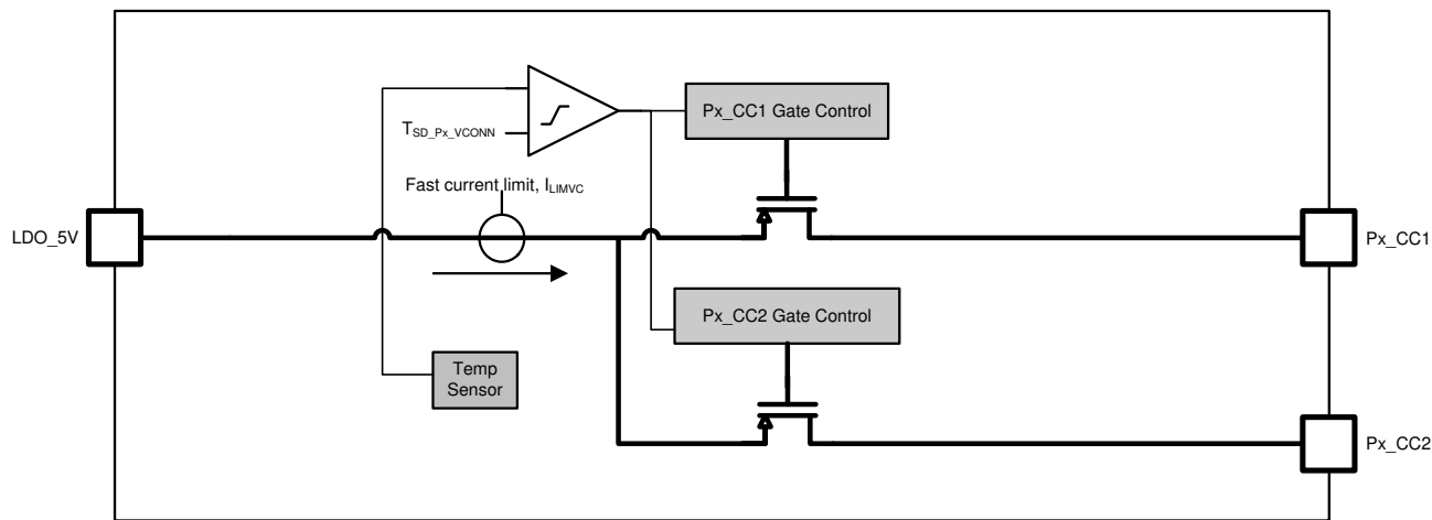
Figure 8-26. VCONN Power Switches
