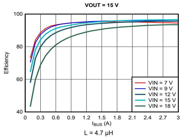
Figure 9-9. Efficiency vs Output Current ( I_{OUT} ), V_{OUT} = 15 V
