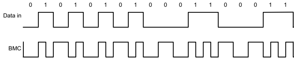
Figure 8-21. Biphase Mark Coding Example
