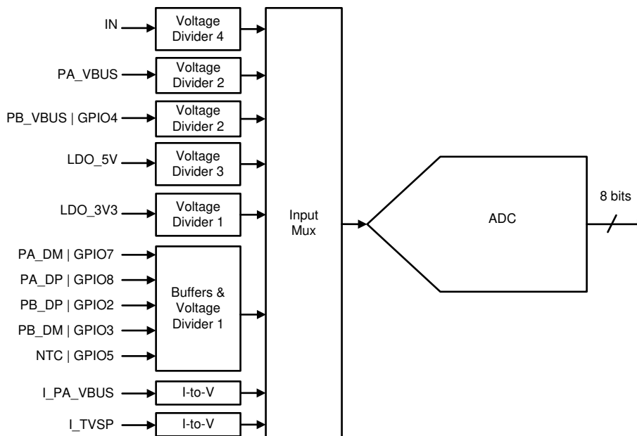
Figure 8-30. SAR ADC
