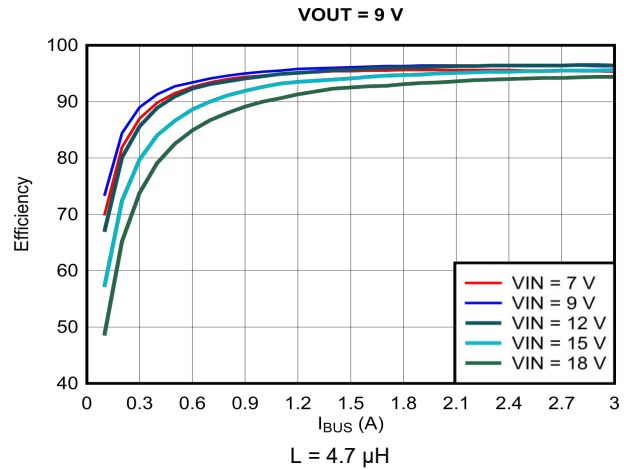
Figure 9-7. Efficiency vs Output Current ( I_{OUT} ), V_{OUT} = 9 V
