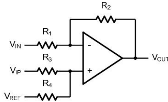
Figure 4. Differential Amplifier
