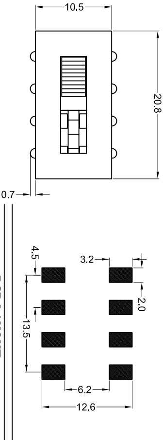
PCB LAYOUT
