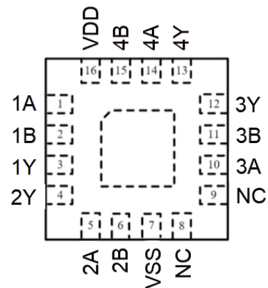
QFN-16 3*3
