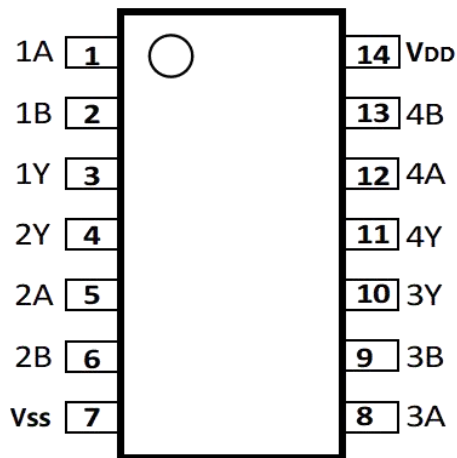
DIP-14/SOP-14/TSSOP-14
