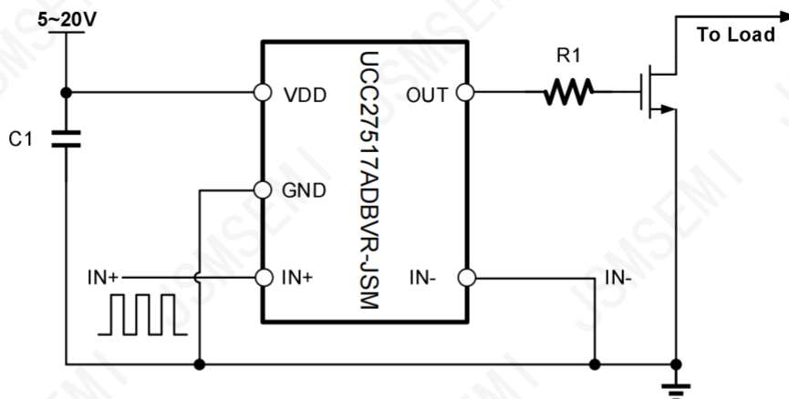
Figure 17 Non-inverting Typical Application Diagram of UCC27517ADBVR-JSM
