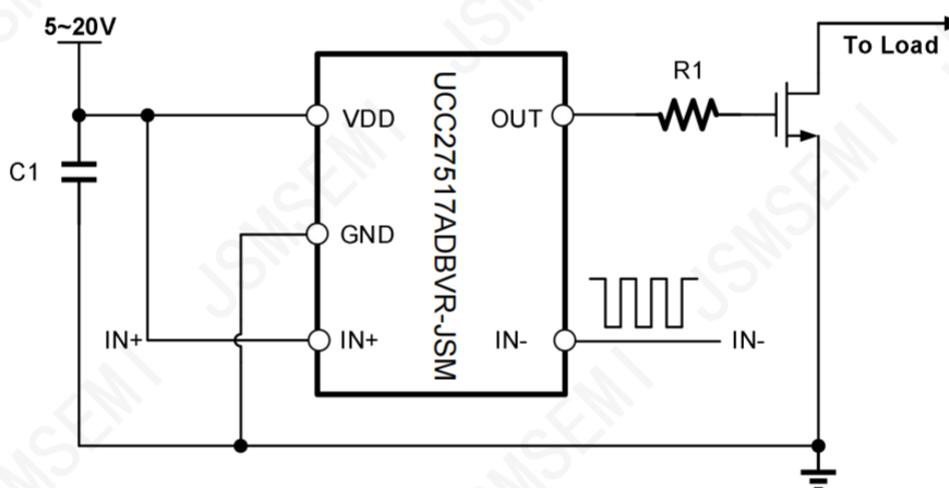
Figure 18 Inverting Typical Application Diagram of UCC27517ADBVR-JSM
