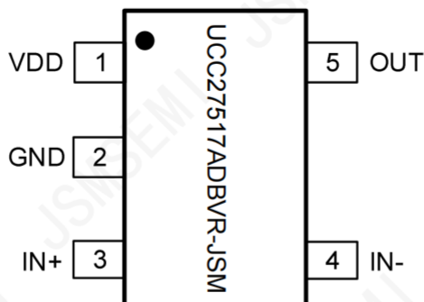
5-Pin SOT-23-5L Package Top View
