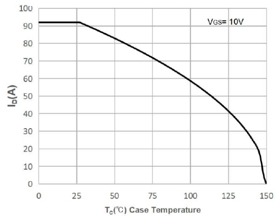
Figure 10: Maximum Continuous Driian Current vs. Case Temperature
