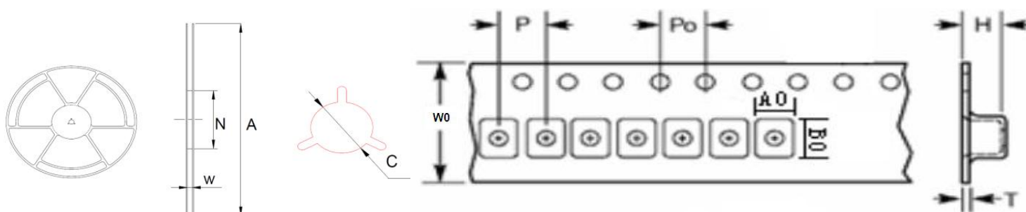
Reel and Taping Dimensions (Unit: mm) Fig:a2
