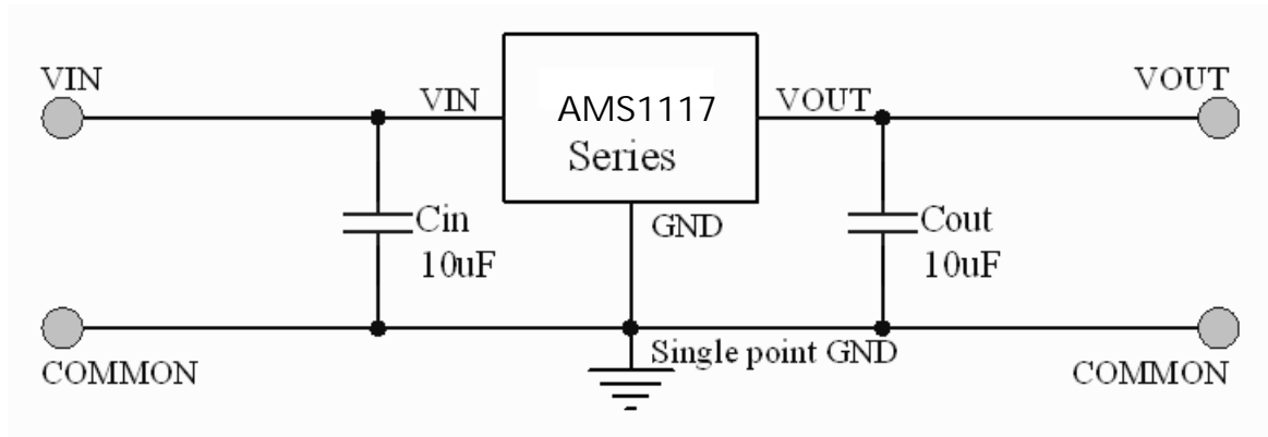
Application circuit of AMS1117 fixed version
