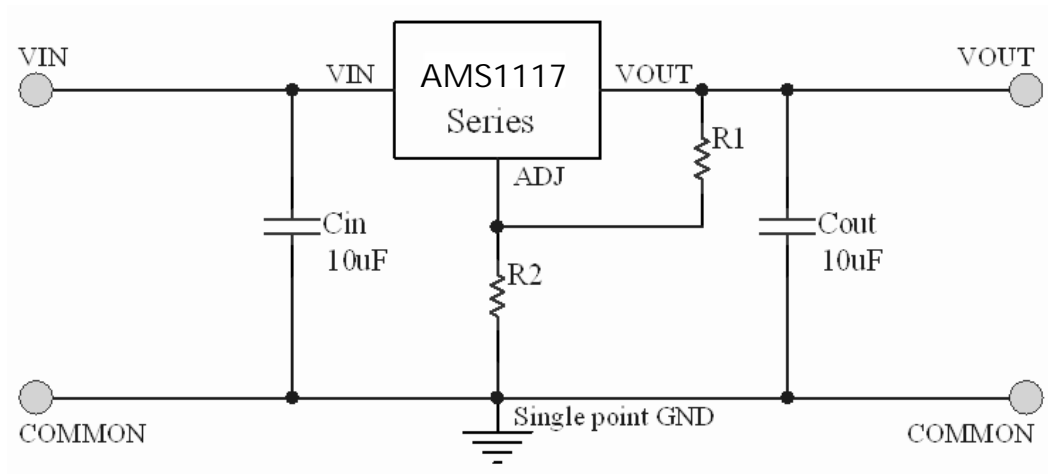
Application Circuit of QN1117-ADJ
