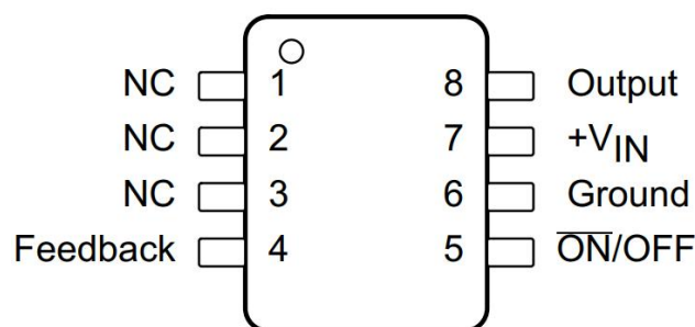
Figure 2.1: SOP8
