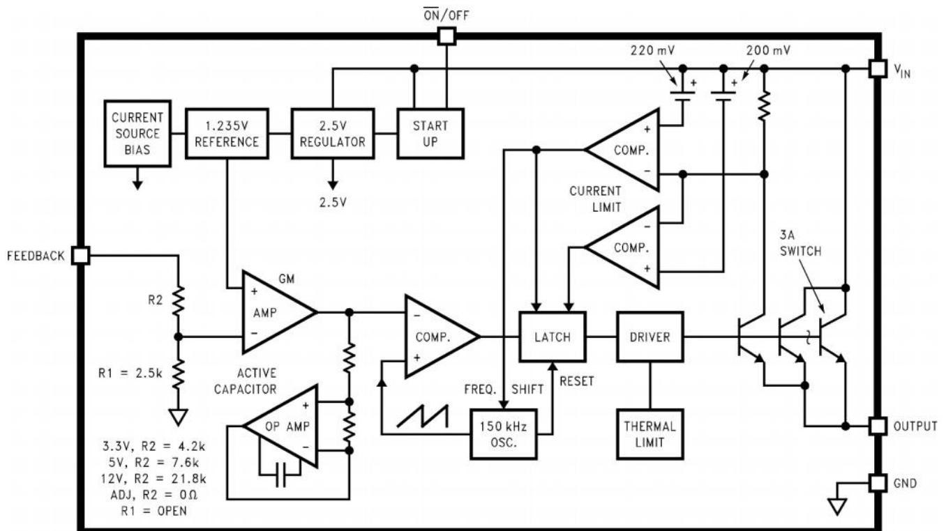
Figure 3.1: LM2594 Functional Block Diagram
