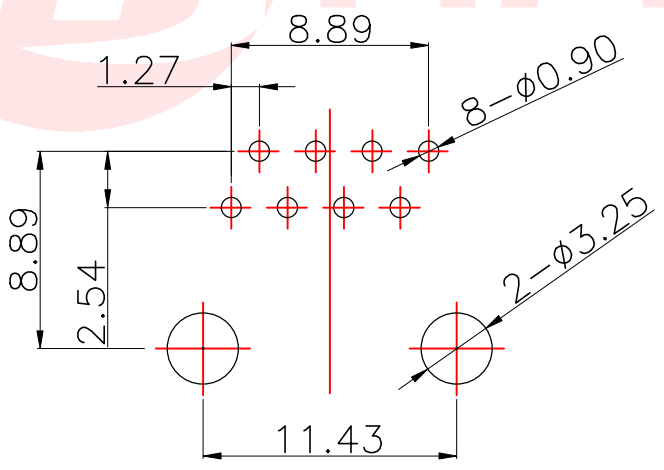
PCB LAYOUT
