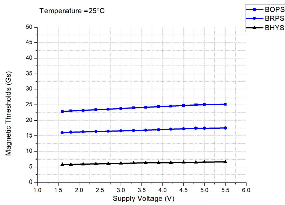
Magnetic Thresholds vs. Supply Voltage @ T_A=25^\circ C
