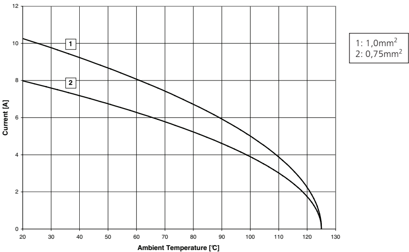
Derating Curve
