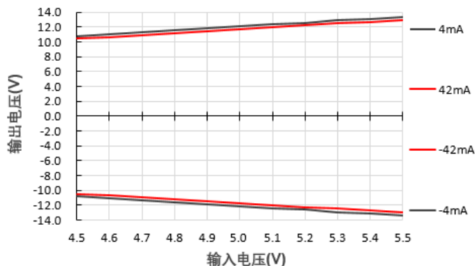
输出电压Vs输入电压@E1205S-1WR3
