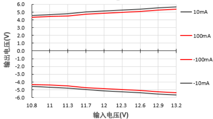
输出电压Vs输入电压@E1205S-1WR3
