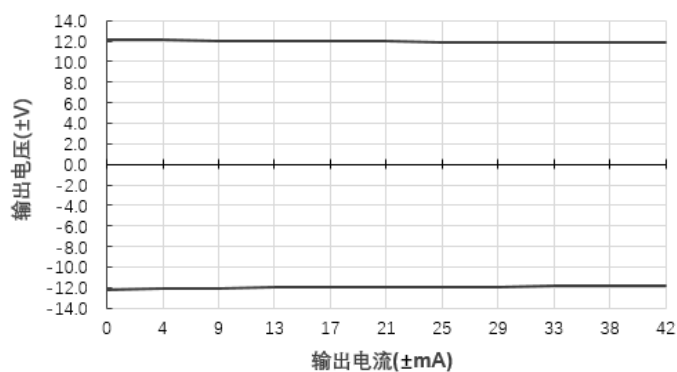
输出电压Vs输出电流(Vin=24V)@E2412S-1WR3
