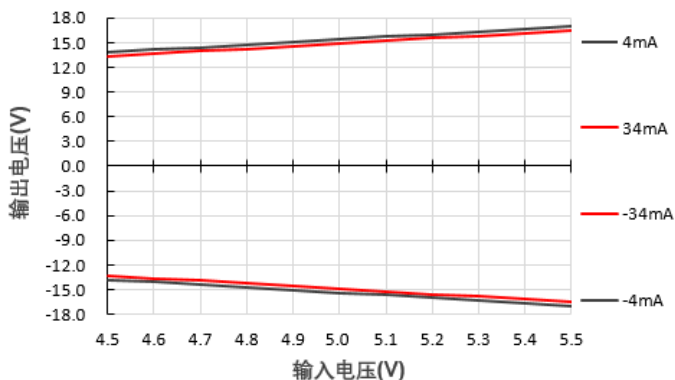
输出电压Vs输入电压@E0515S-1WR3
