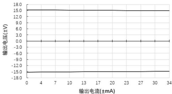
输出电压Vs输出电流(Vin=12V)@E1215S-1WR3
