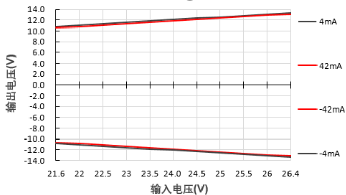
输出电压Vs输入电压@E2412S-1WR3
