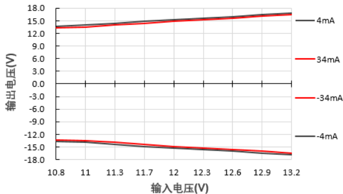
输出电压Vs输入电压@E1215S-1WR3
