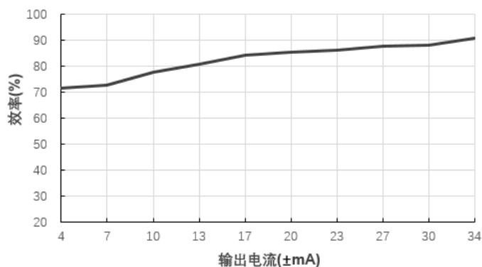
效率Vs输出电流(Vin=24V)@E2415S-1WR3
