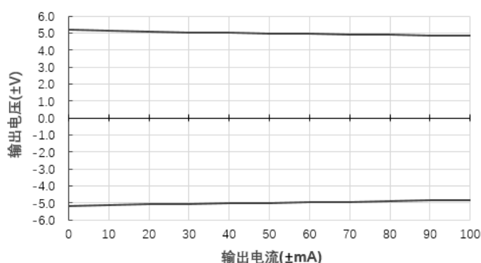
输出电压Vs输出电流(Vin=12V)@E1205S-1WR3
