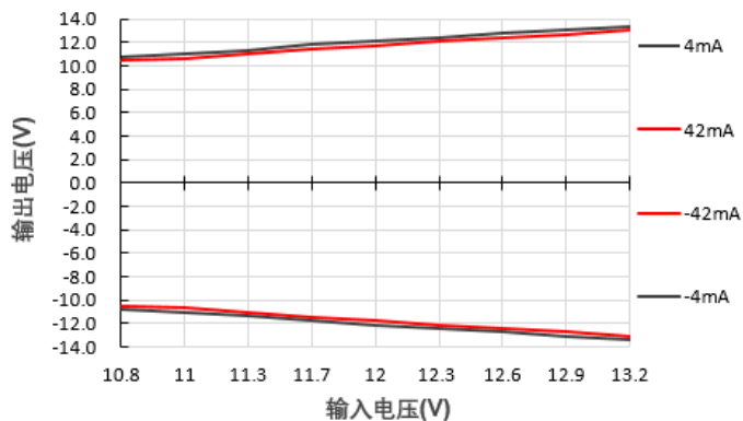
输出电压Vs输入电压@E2405S-1WR3
