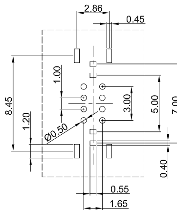
PCB REFERENCE DIAGRAM TOLERANCE:±0.05
