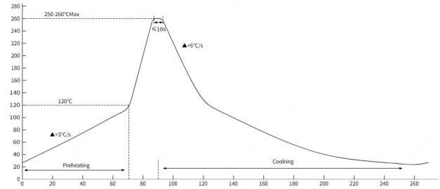
波峰焊 Wave-Soldering Profile
