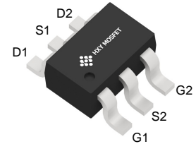
SOT-23-6L (TSOP-6-1.5mm)
