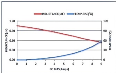
ZEP1M404010S-1R0M
