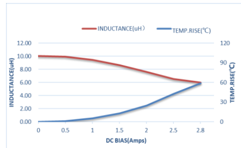
ZEP1M404010S-100M
