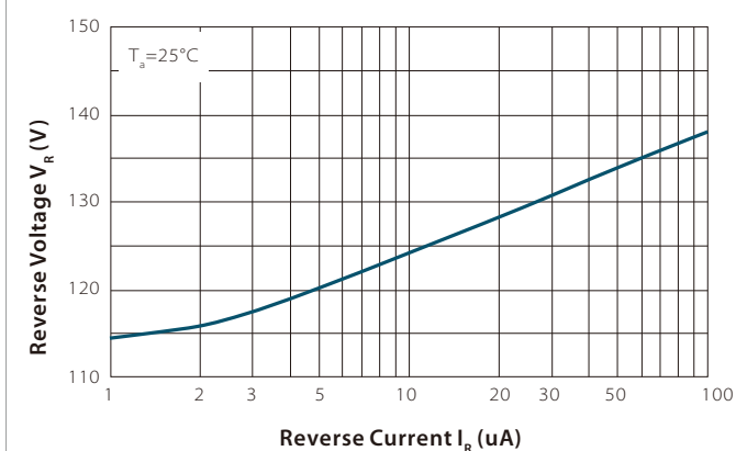
Fig 1. Reverse Voltage vs Reverse Current BV-1.0 to 100uA
