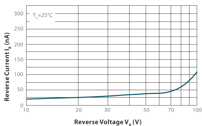
Fig 2. Reverse Current vs Reverse Voltage IR-10 to 100V
