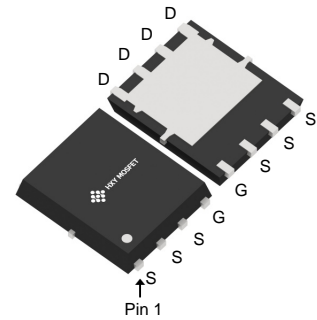
DFN5X6-8L (TDSON-8-EP(5.1x5.9))
