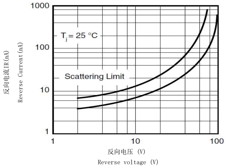
反向特性曲线 (典型值) Typical Reverse Characteristics
