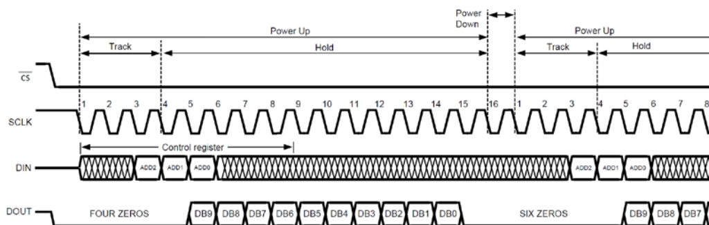
Figure 4. Timing Diagram
