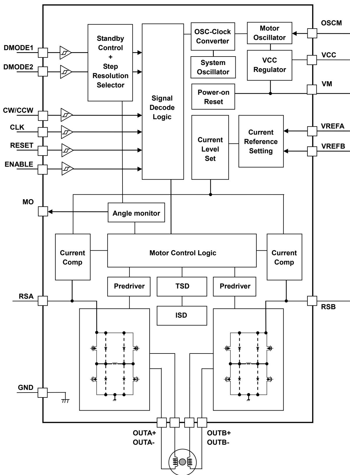
TB67S102A Block diagram
