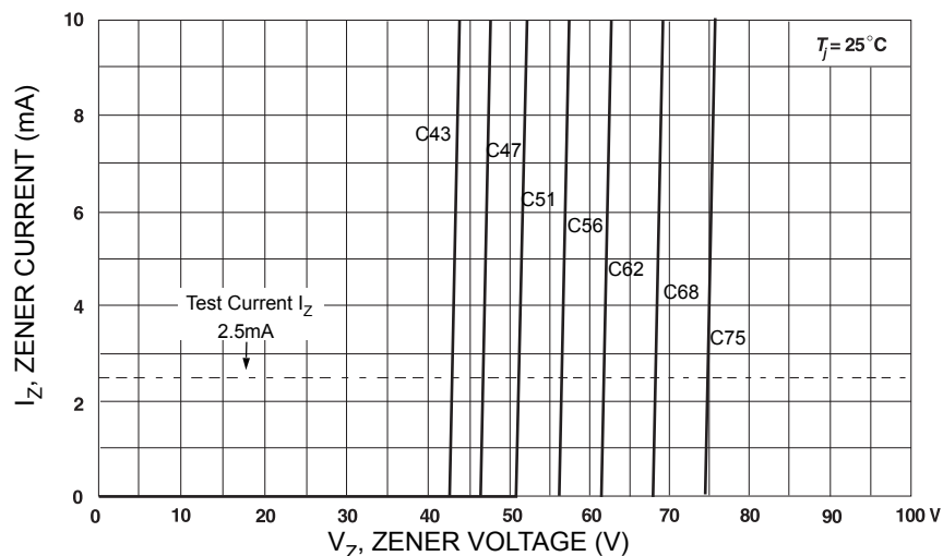
Fig. 5 Zener Breakdown Characteristics
