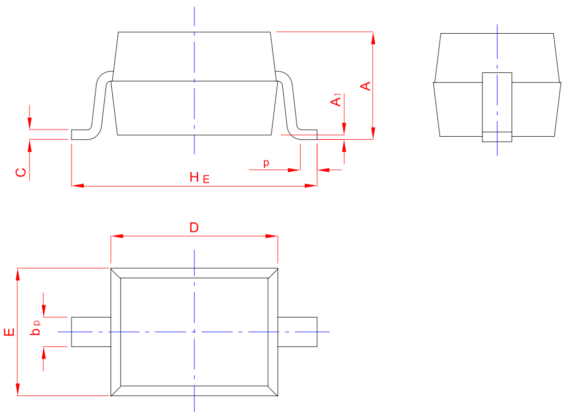
SOD-323
