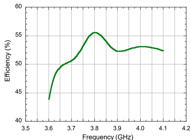
Efficiency vs. Frequency, 2.5dB Gain Compression
