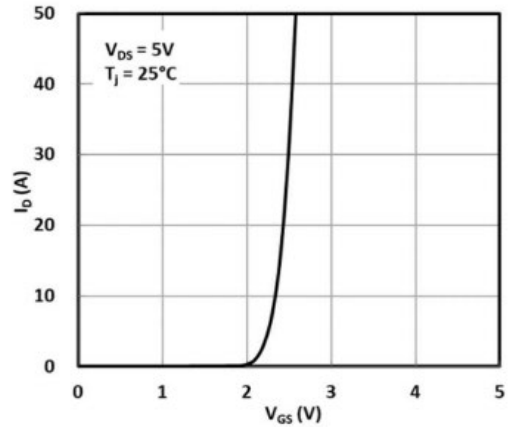
Fig. 2 Transfer characteristics
