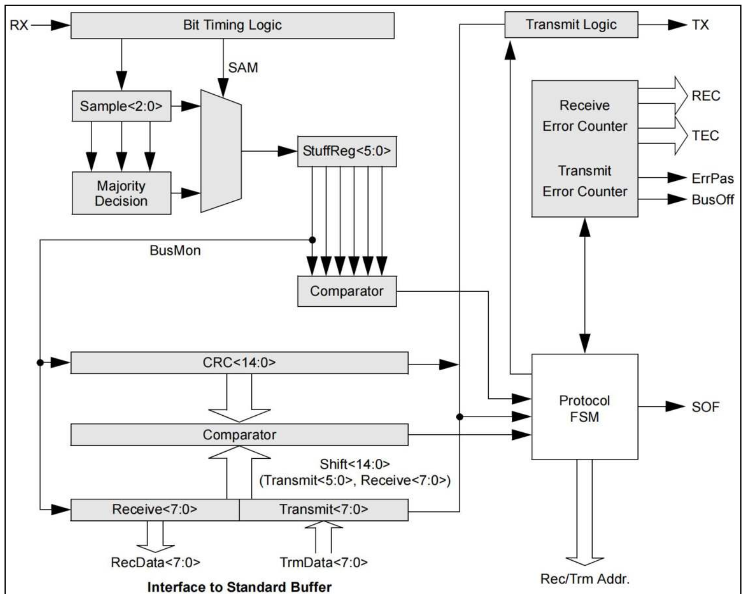
FIGURE 3: CAN PROTOCOL ENGINE BLOCK DIAGRAM
