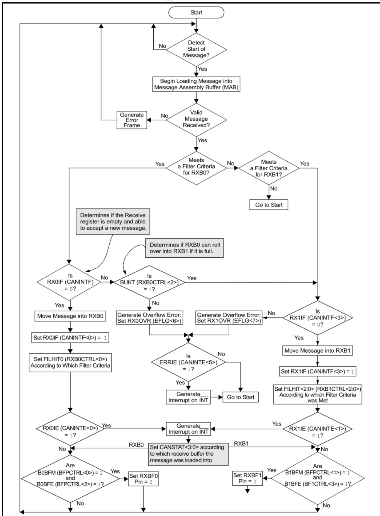
FIGURE 13: RECEIVE FLOWCHART
